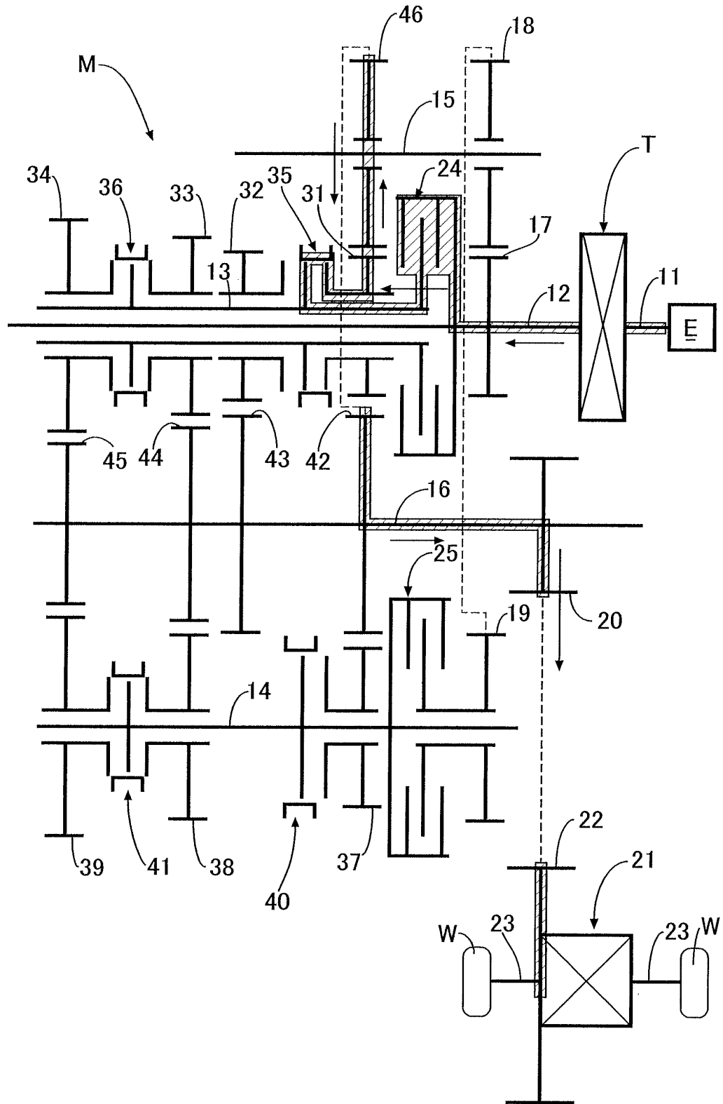
FIG.67 REVERSE GEAR POSITION (RVS)
