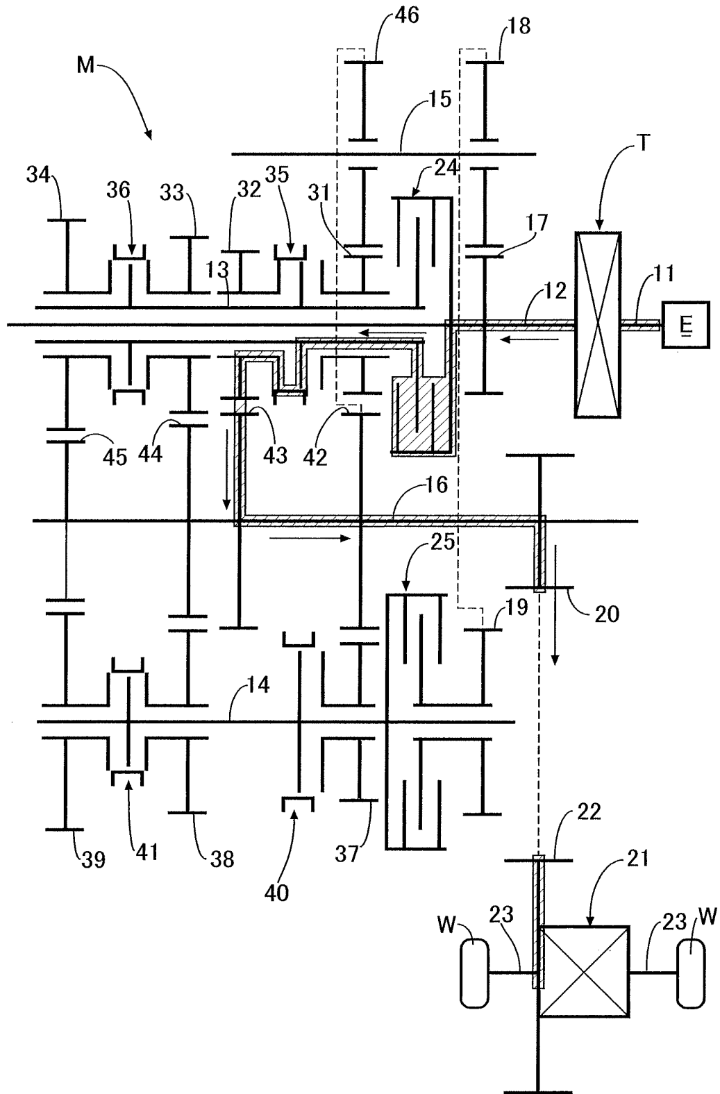
FIG.62 SECOND SPEED GEAR POSITION (2ND)
