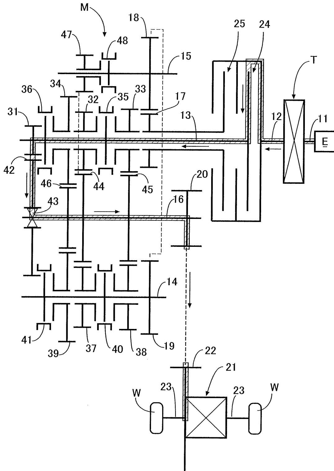
FIG.71 FIRST SPEED GEAR POSITION (LOW)
