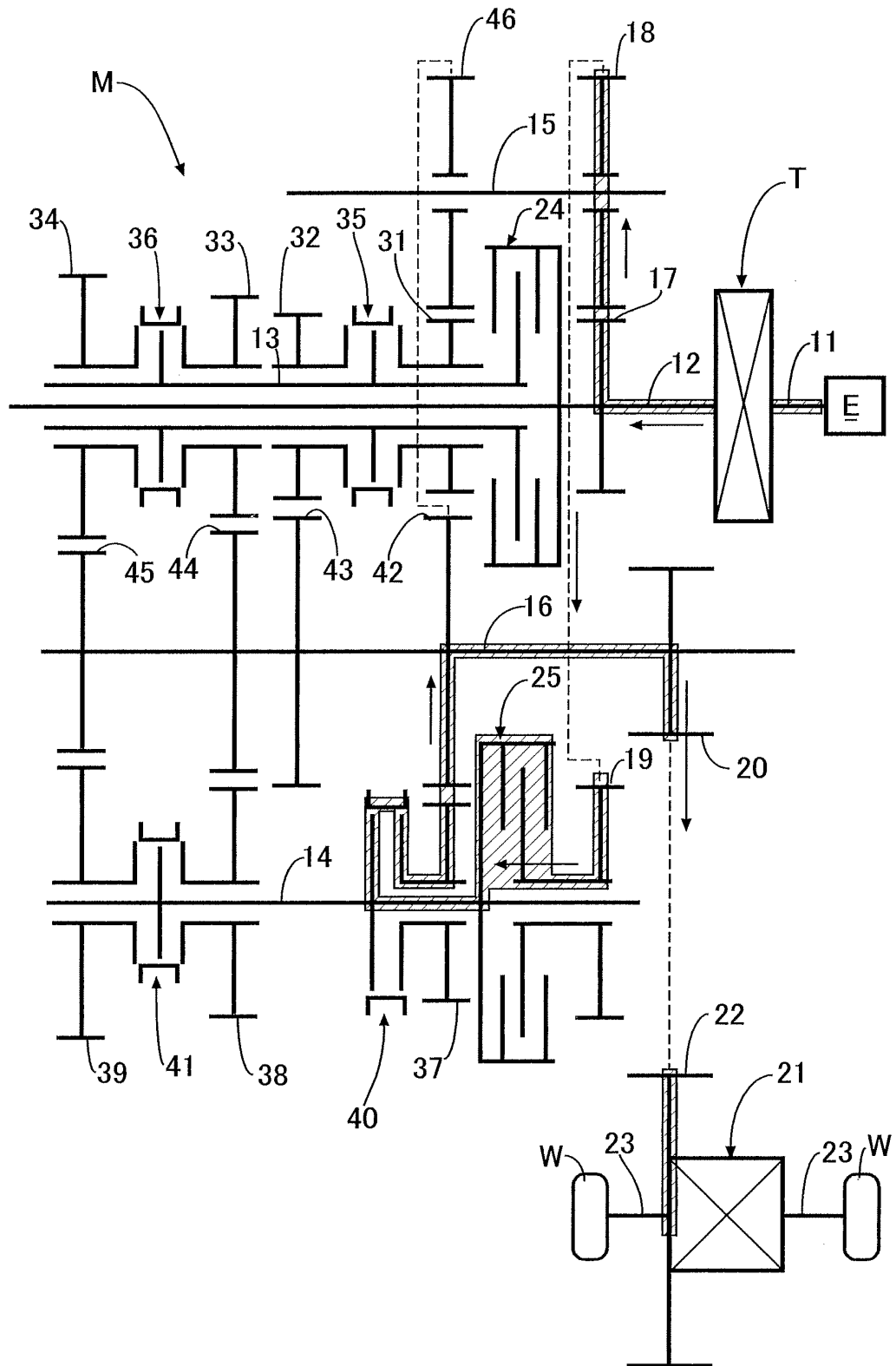
FIG.61 FIRST SPEED GEAR POSITION (LOW)
