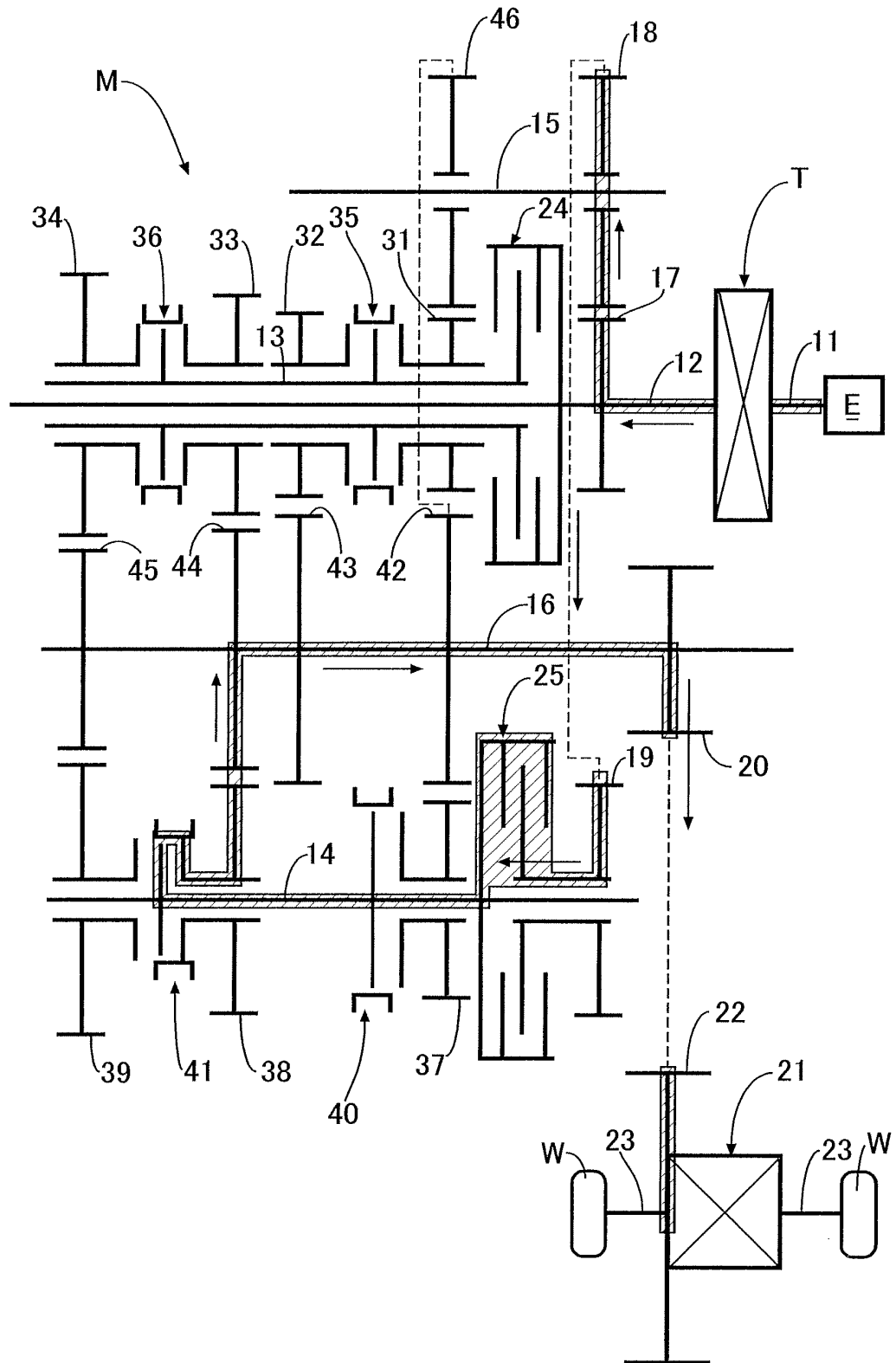
FIG.63 THIRD SPEED GEAR POSITION (3RD)
