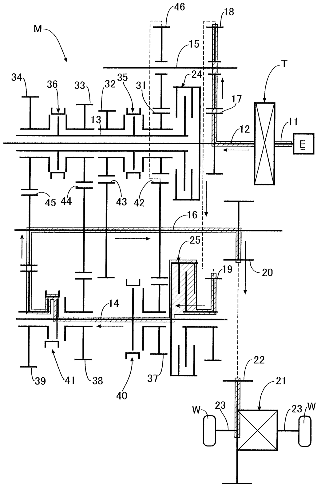
FIG.65 FIFTH SPEED GEAR POSITION (5TH)
