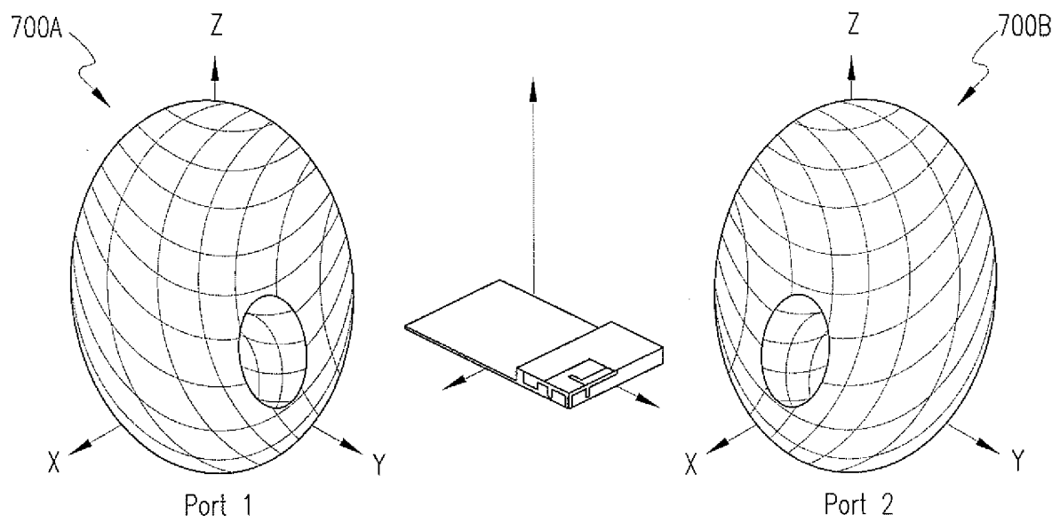
Measured antenna 3D radiation pattern at 2.45 GHz
