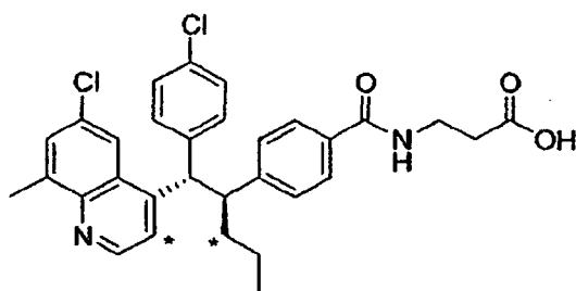
Diastereomer A
