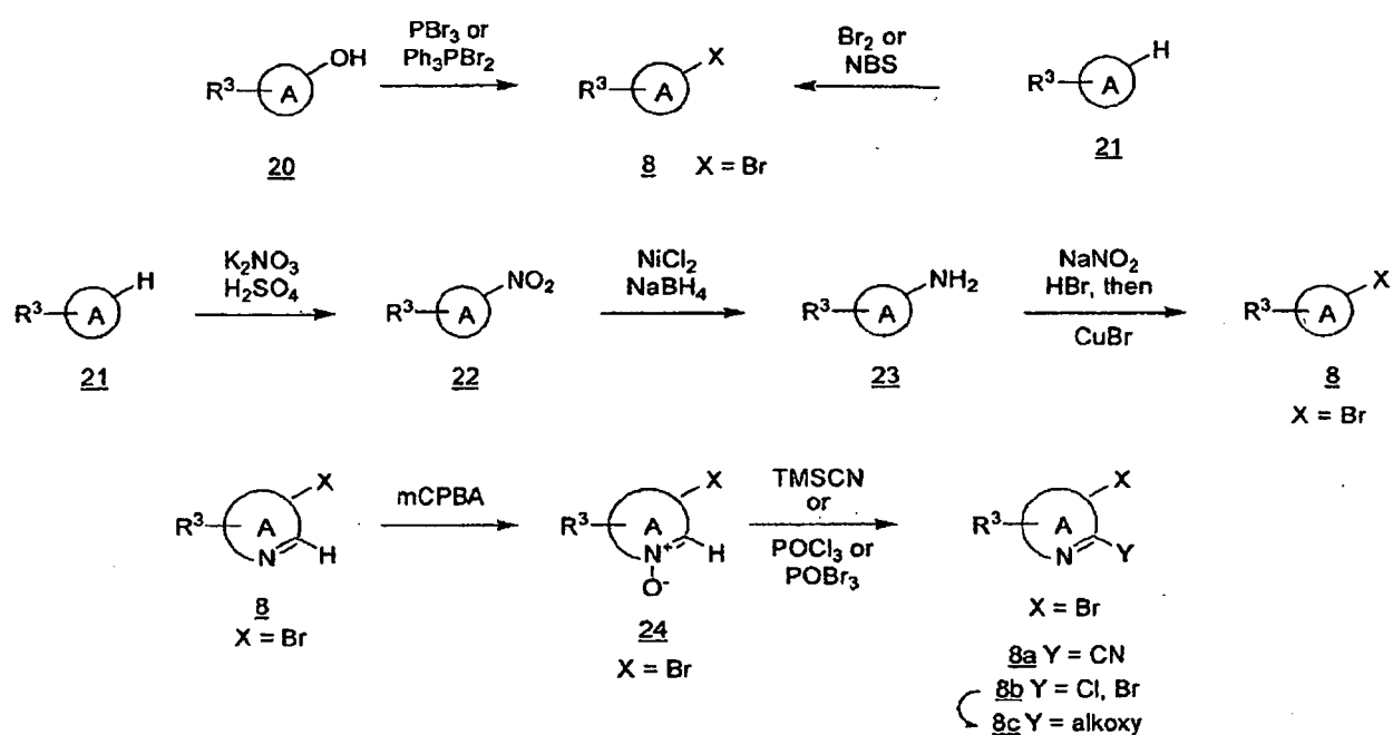
Scheme 8
