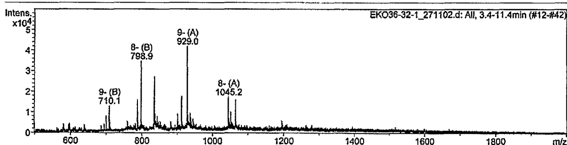
All, 3.4-11.4min (#12-#42)
