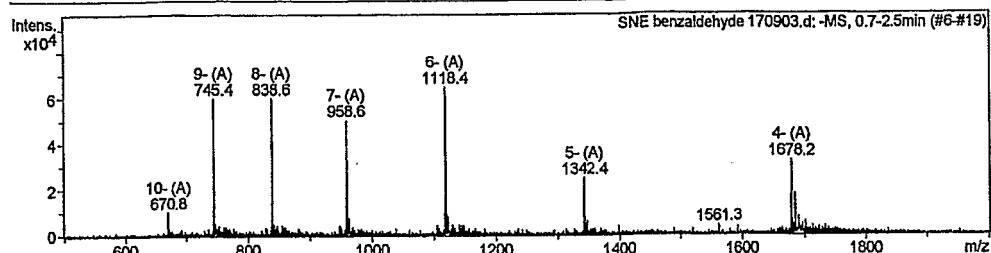
-MS, 0.7-2.5min (#6-#19)
