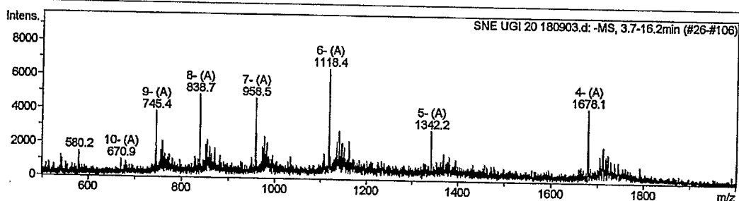
-MS, 3.7-16.2min (#26-#106)
