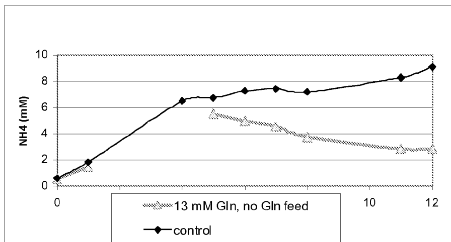
Figure 5. Ammonium levels of anti-GDF-8 cell cultures in control and no glutamine feed culture conditions.
