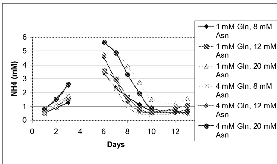
Figure 33. Ammonium levels of anti-GDF-8 cultures under various experimental conditions.
