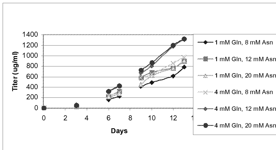
Figure 31. Anti-GDF-8 titer under various experimental conditions.
