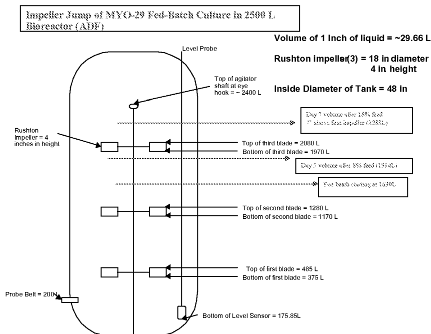
Figure 24. Impeller Jump
