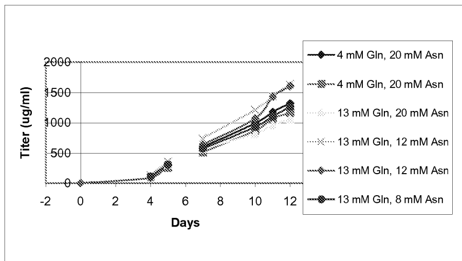
Figure 39. Anti-GDF-8 titer in modified Medium 9 containing various levels of glutamine and asparagine.
