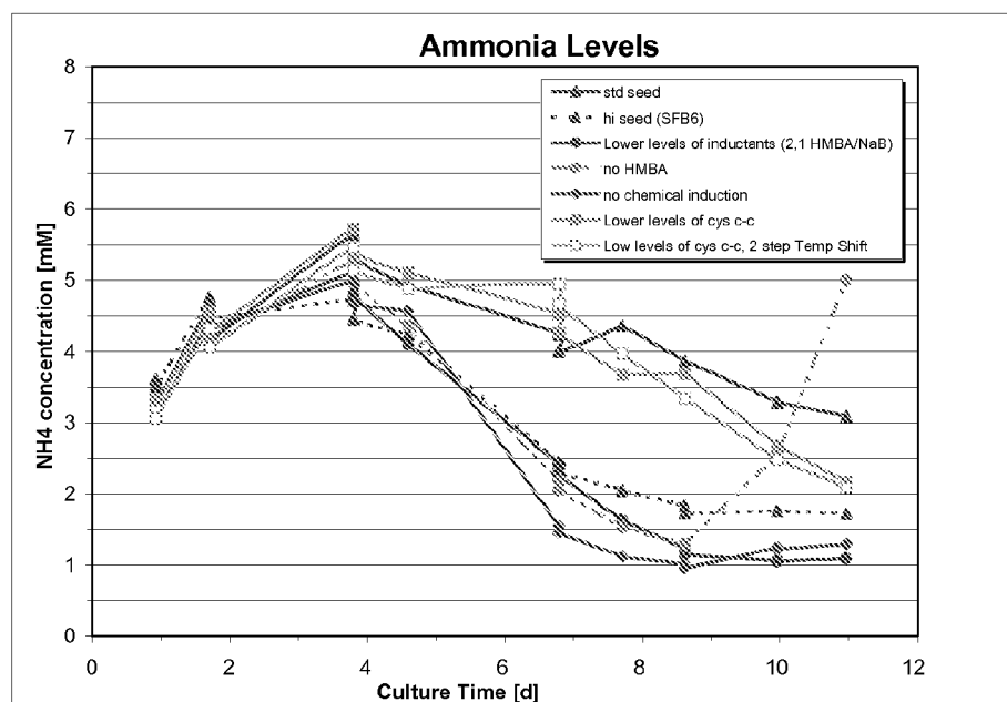
Figure 71. Ammonium levels in cultures of cells expressing TNFR-Ig under various experimental conditions.
