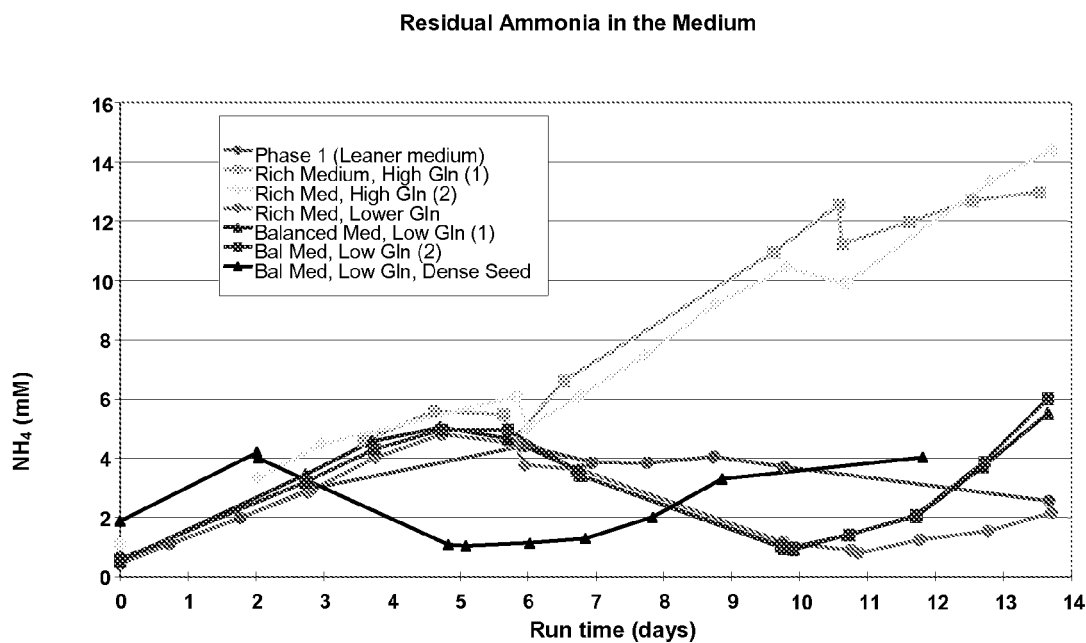
Figure 63. Ammonium levels of anti-ABeta cultures under various media conditions tested.
