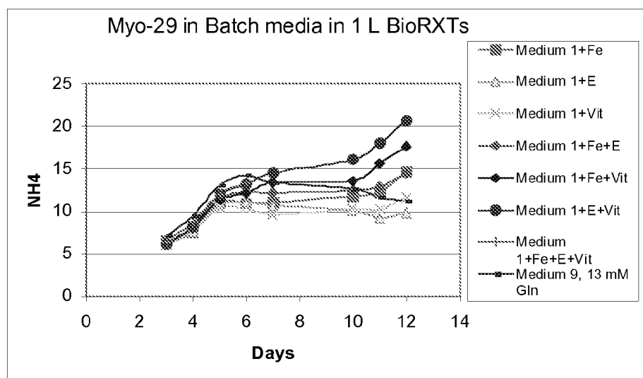
Figure 55. Ammonium levels of anti-GDF-8 cultures in media containing various levels of vitamins, trace elements E and iron.
