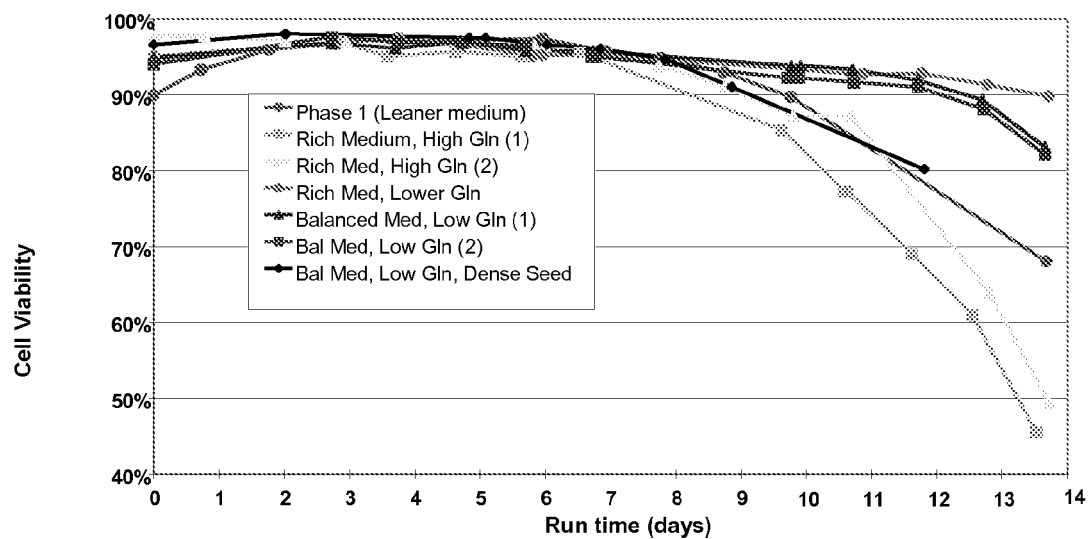
Figure 61. Viability of anti-ABeta cells under various media conditions tested.
