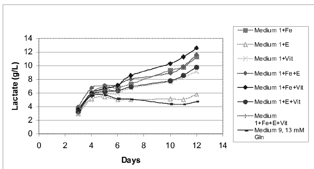
Figure 54. Lactate levels of anti-GDF-8 cultures in media containing various levels of vitamins, trace elements E and iron.
