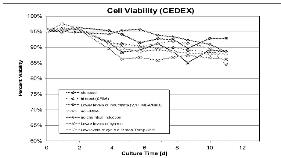
Figure 67. Viability of cells expressing TNFR-Ig under various experimental conditions.
