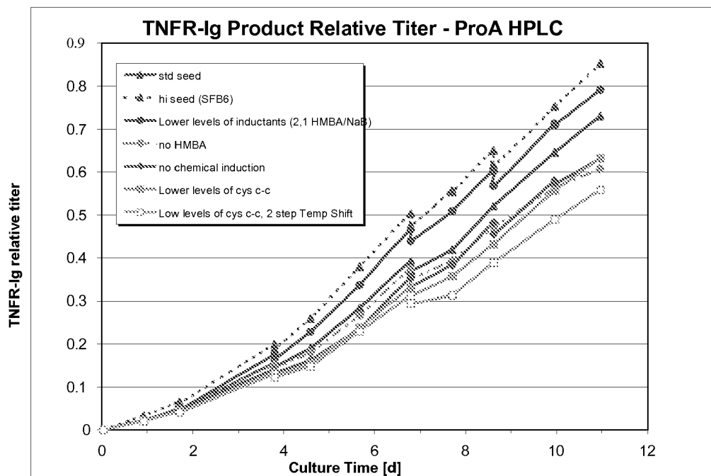
Figure 72. TNFR-Ig relative titer under various experimental conditions.
