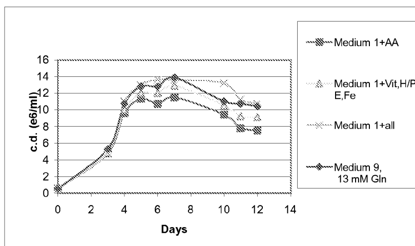
Figure 48. Cell growth of anti-GDF-8 cells in media containing various levels of amino acids and vitamins.
