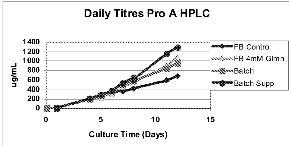
Figure 27. Anti-GDF-8 titer under various experimental conditions.
