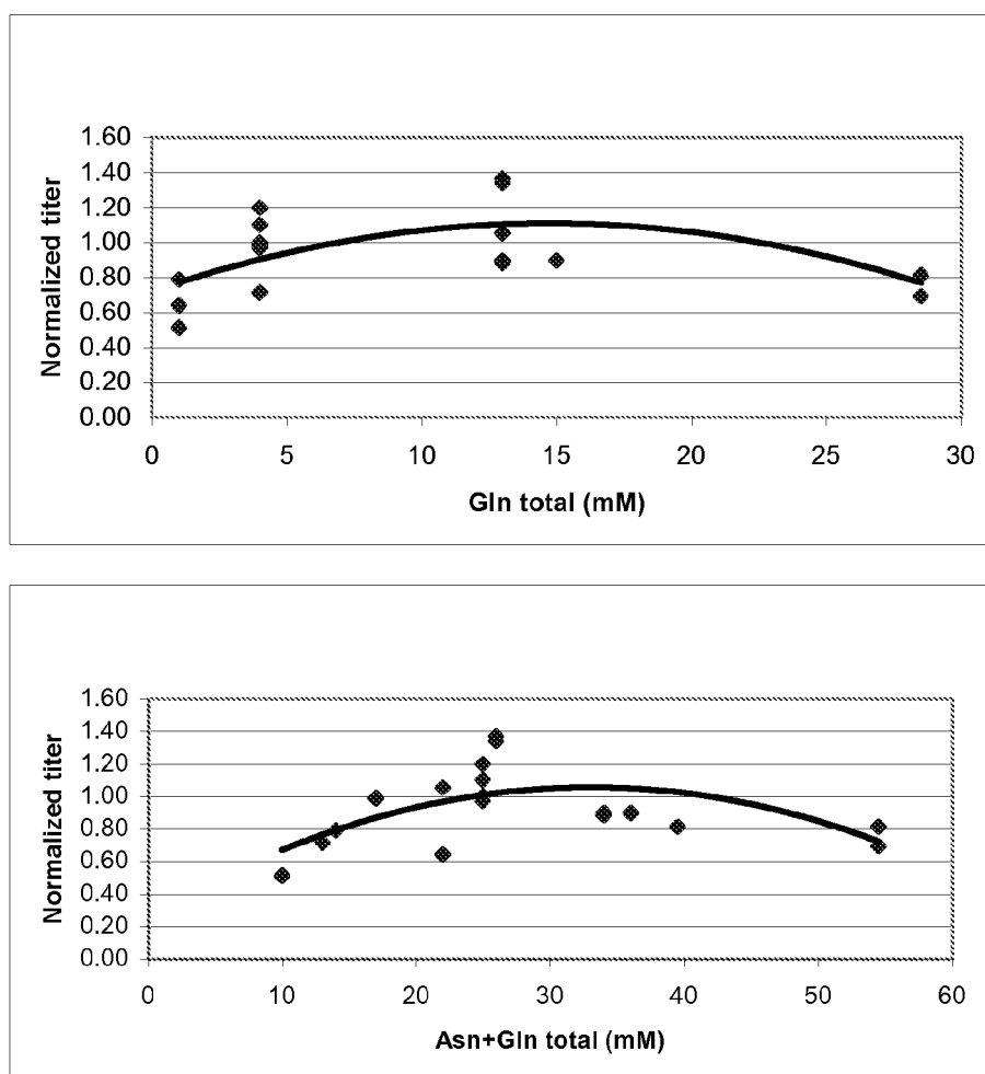
Figure 59. Extrapolated anti-GDF-8 titers for various levels of glutamine alone and total combined glutamine and asparagine.
