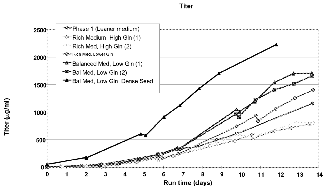
Figure 64. Anti-ABeta titer in various media conditions tested.
