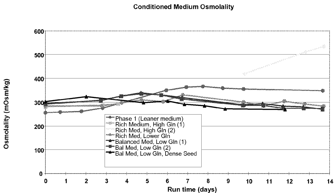
Figure 65. Osmolarity of anti-ABeta cultures under various media conditions tested.
