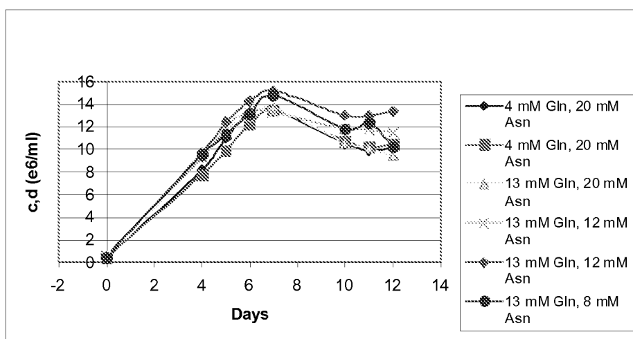
Figure 34. Cell growth of anti-GDF-8 cells in modified Medium 9 containing various levels of glutamine and asparagine.
