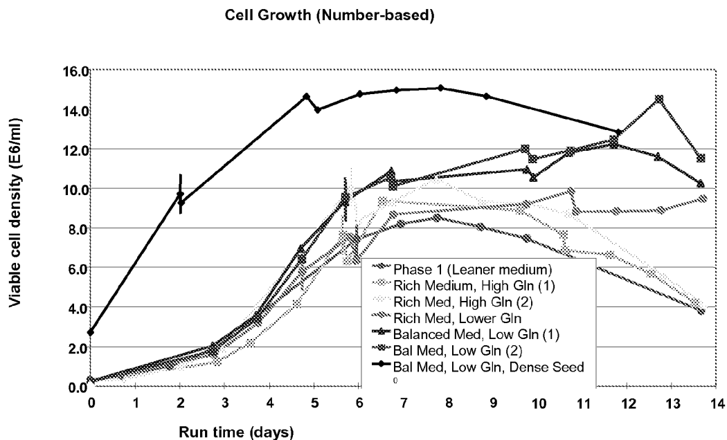
Figure 60. Growth of anti-ABeta cells under various media conditions tested.
