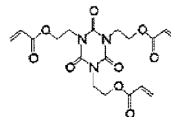
Monomer C
