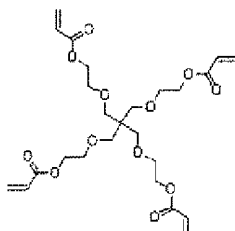
Monomer B
