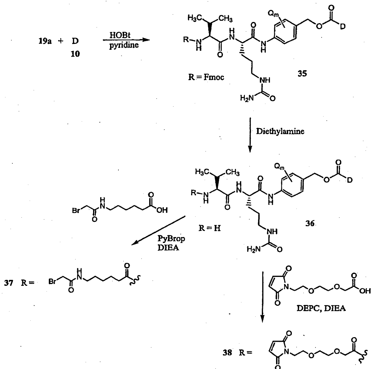
Scheme 14
