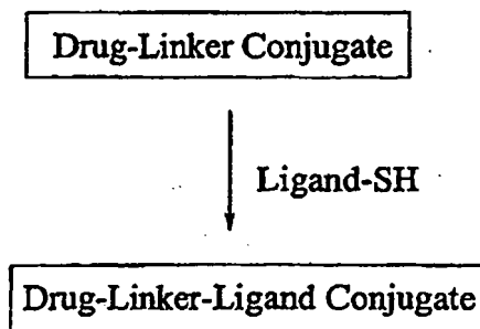
Scheme 17
