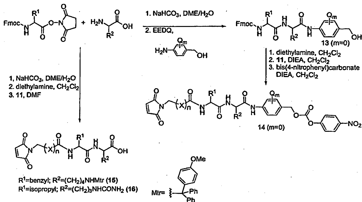
Scheme 10
