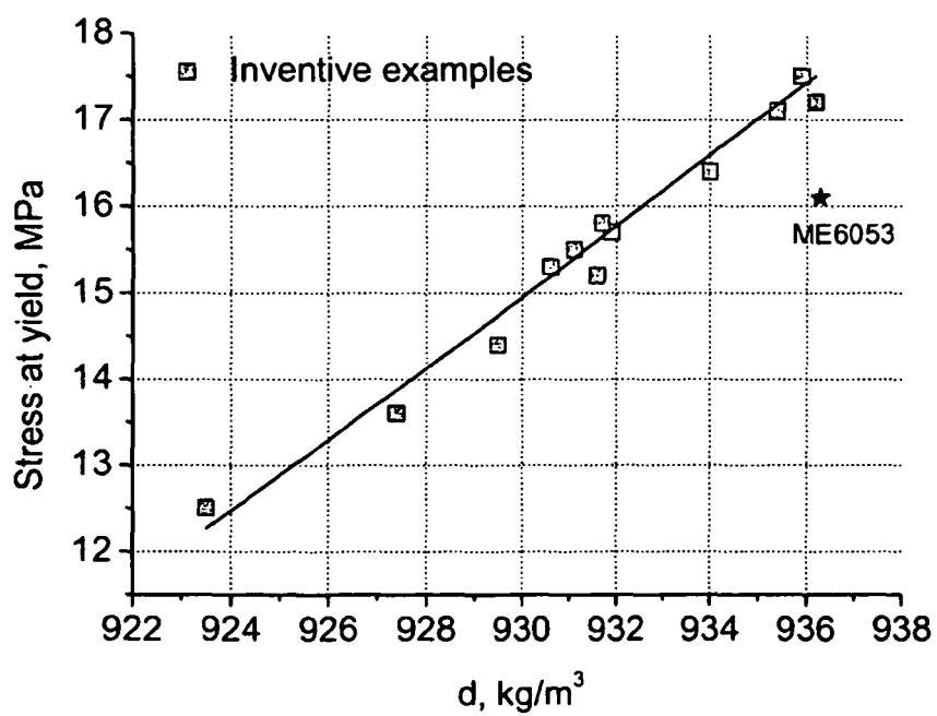
Figure 2. Stress at yield vs. density.
