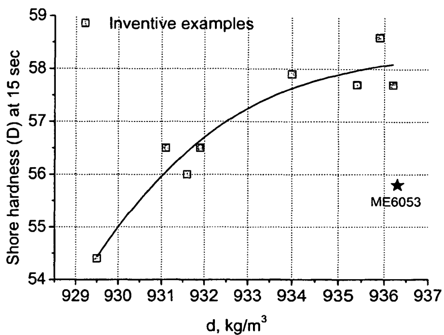
Figure 3. Shore D hardness (ASTM D2240-05) at 15 seconds vs. density for the inventive examples and ME6053
