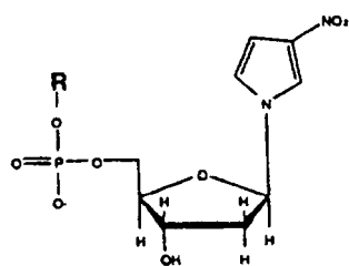
3-nitropyrrole
