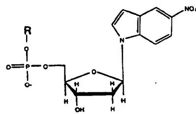
5-nitroindole
