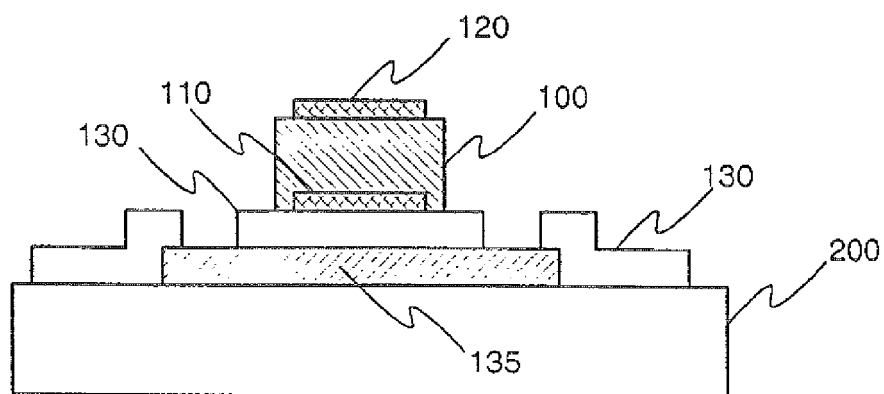
Fig. 3 PRIOR ART
