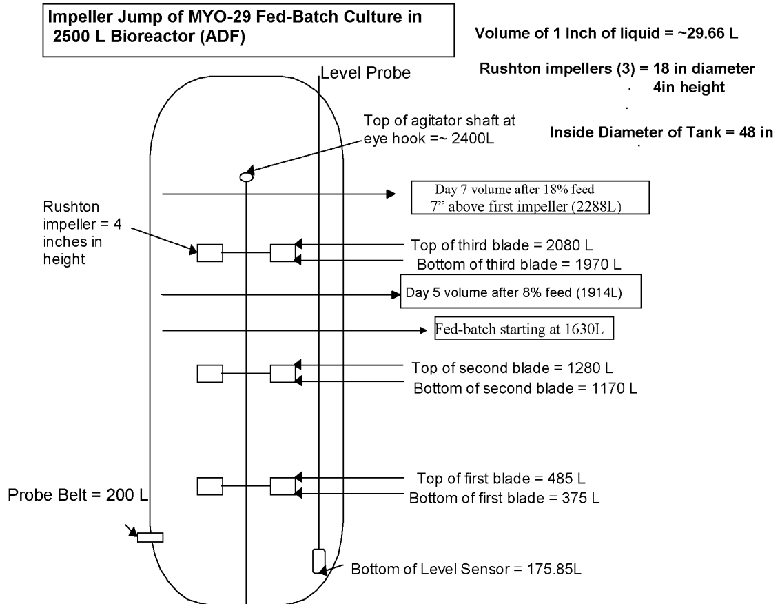
Figure 24. Impeller Jump
