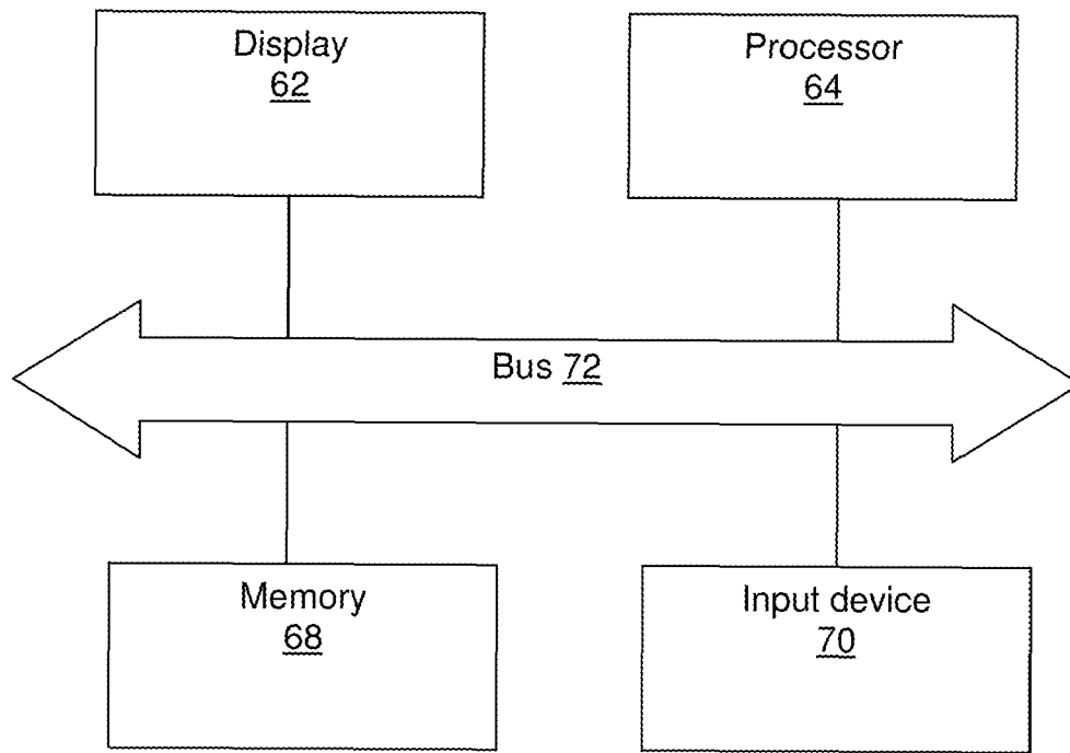
Computing Device 60
