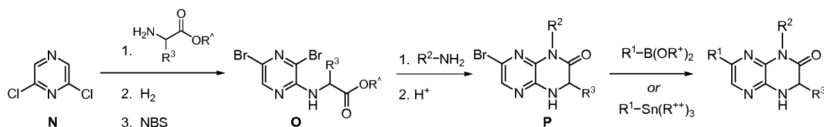
Scheme 8
