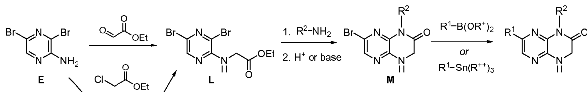
Scheme 7
