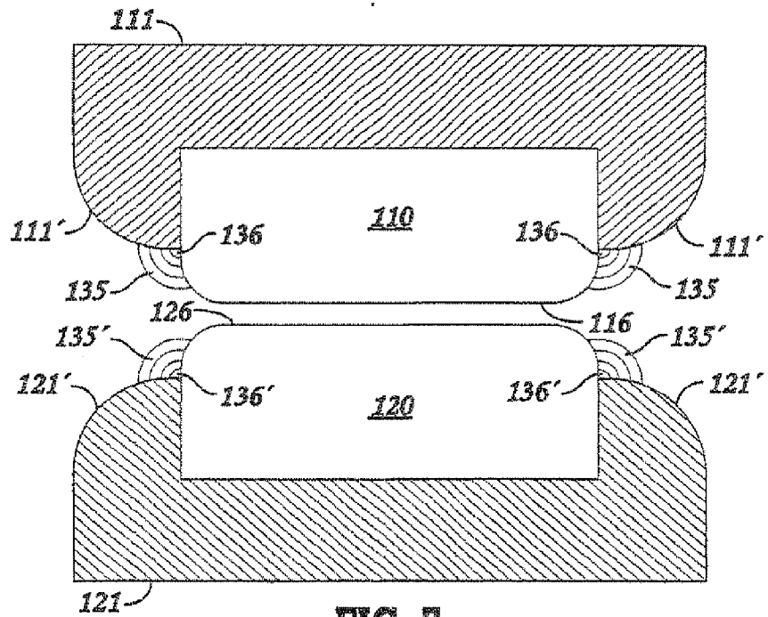
FIG. 7 (Prior Art)
