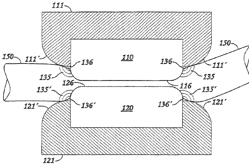
FIG. 8 (Prior Art)
