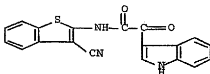
75) 1H-Indole-3-acetamide, N-(3-cyanobenzo[b]thien-2-yl)-α-oxo-
