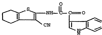
78) 1H-Indole-3-acetamide, N-(3-cyano-4,5,6,7-tetrahydrobenzo[b]thien-2-yl)-α-oxo-
