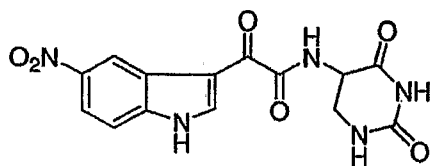
97) N-(2,4-dioxo-1,2,3,4-tetrahydropyrimidin-5-yl)-2-(5-nitro-1H-indol-3-yl)-2-oxo-acetamide
