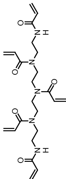
Polymerizable compound 36
