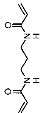
Polymerizable compound 7
