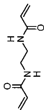
Polymerizable compound 1
