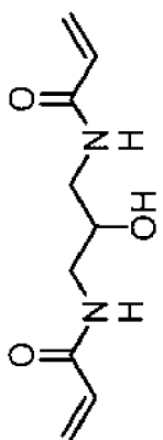
Polymerizable compound 9
