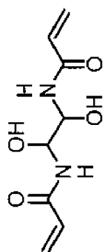
Polymerizable compound 10
