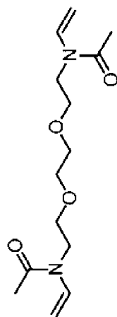
Polymerizable compound 6
