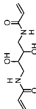
Polymerizable compound 13
