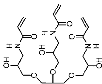
Polymerizable compound 22 A value: 157.8
