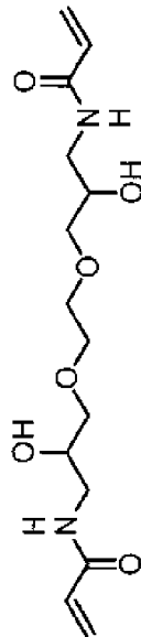
Polymerizable compound 14
