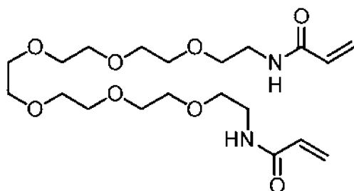
Comparative Polymerizable Compound 2 A value: 216.3
