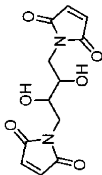
Polymerizable compound 27 A value: 140.1
