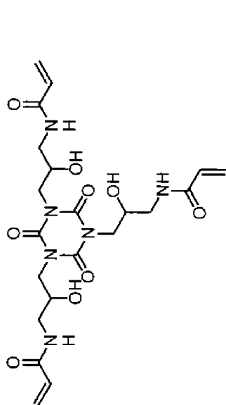
Polymerizable compound 16 A value: 170.2
