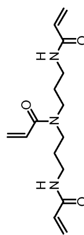
Polymerizable compound 37 A value: 97.8
