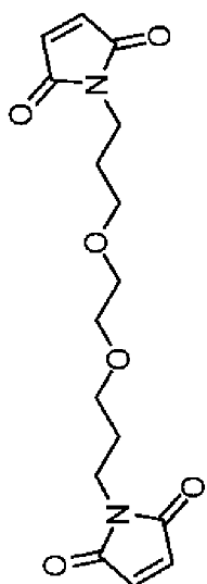
Polymerizable compound 26 A value: 168.2
