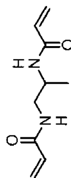
Polymerizable compound 8
