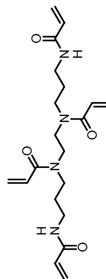
Polymerizable compound 39 A value: 97.6
