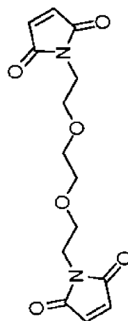
Polymerizable compound 24 A value: 154.1
