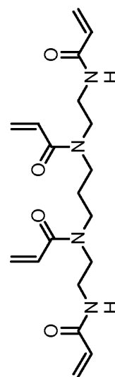
Polymerizable compound 40 A value: 94.1
