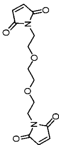
Polymerizable compound 4
