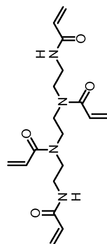
Polymerizable compound 35
