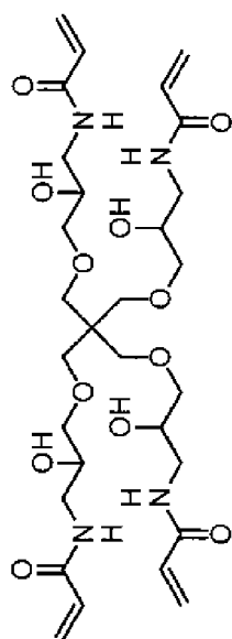
Polymerizable compound 21 A value: 161.2
