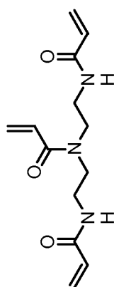
Polymerizable compound 34 A value: 88.4
