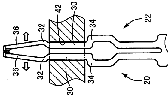
FIG. 4D COMPLETION OF INSERTION OF SUBSTRATE
