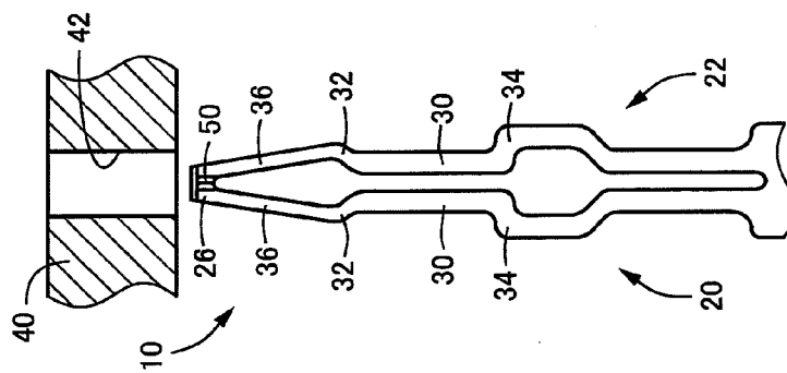
FIG. 4A BEFORE INSERTION OF SUBSTRATE
