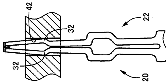
FIG. 4C DURING INSERTION OF SUBSTRATE
