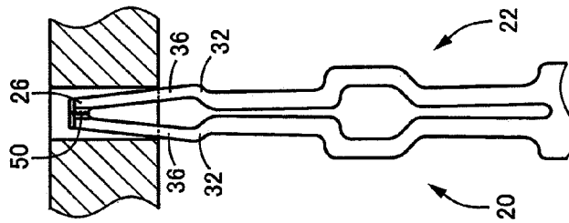
FIG. 4B BREAKAGE OF DISTAL END PORTION
