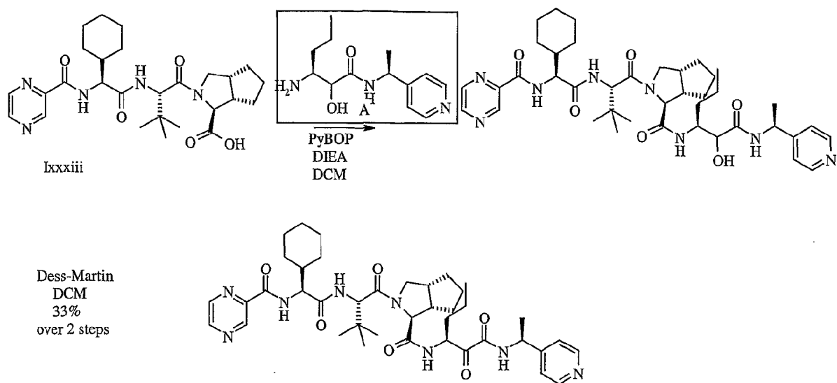
Scheme 9
