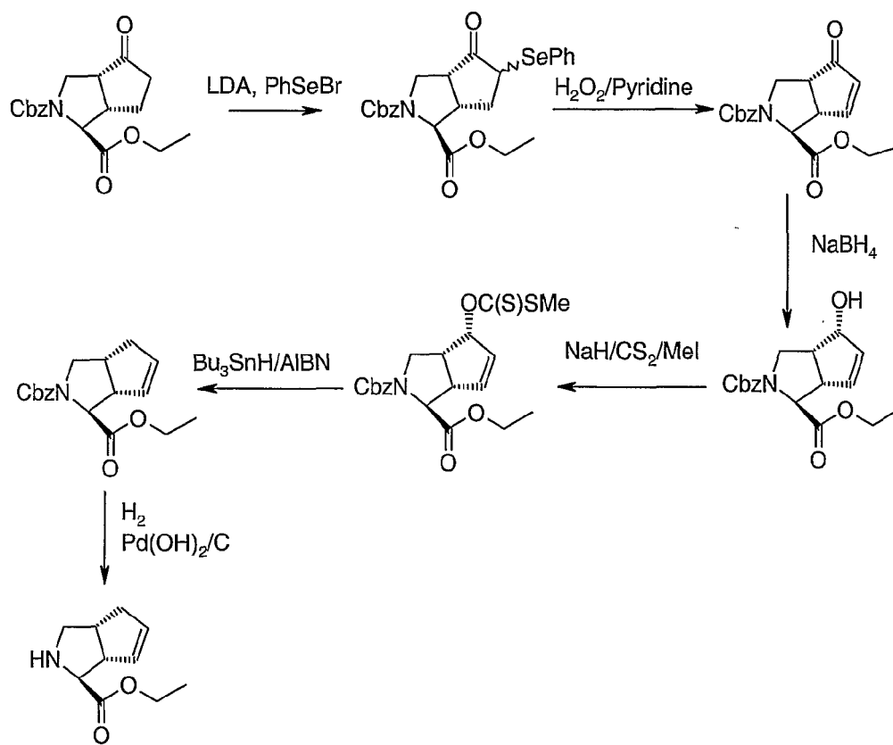
SCHEME 3
