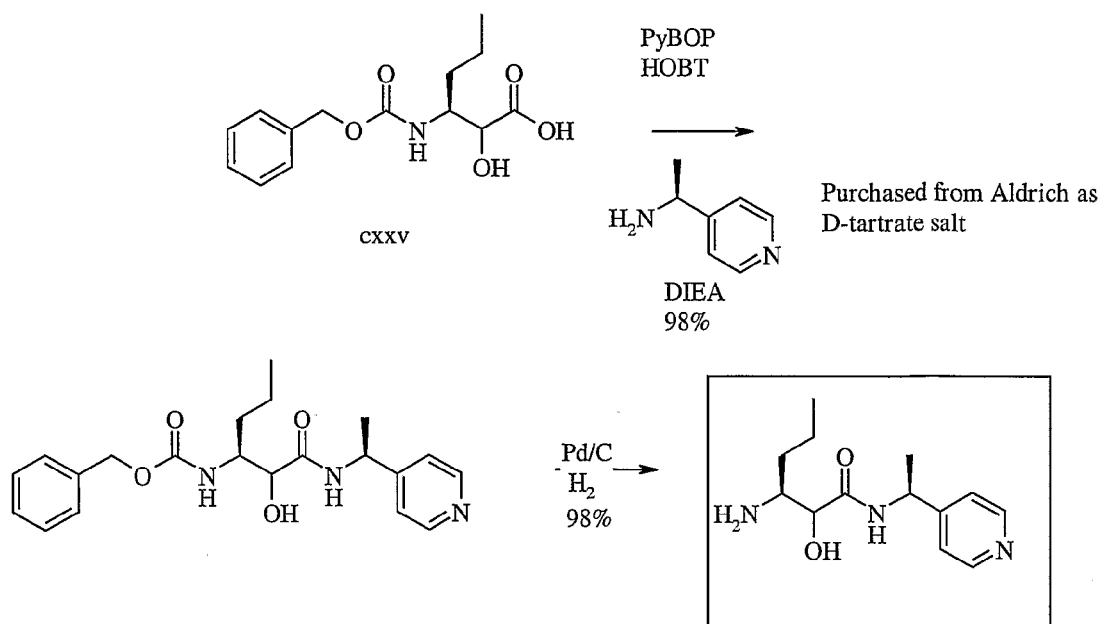
SCHEME 10
