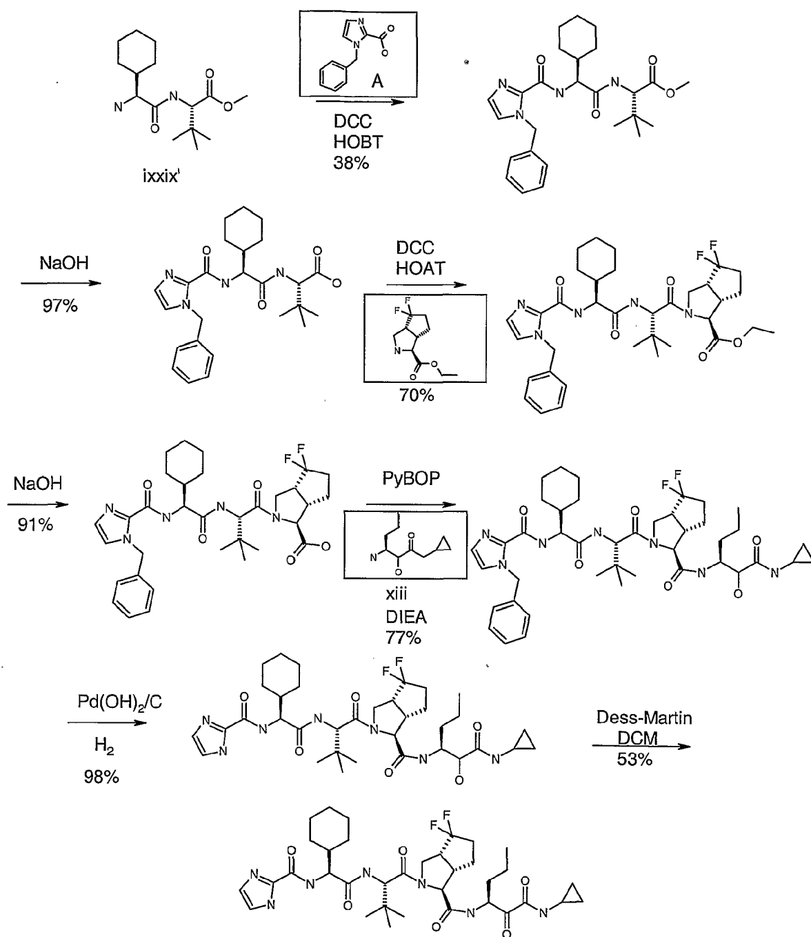
Scheme 11
