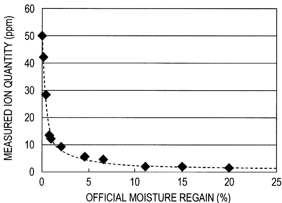
MEASURED ION QUANTITY OF SHIELDING MEMBER AT 1 MILLION SHEETS FOR DURABILITY TEST
