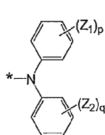
Formula 6A
