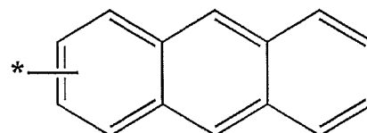
Formula 5C
