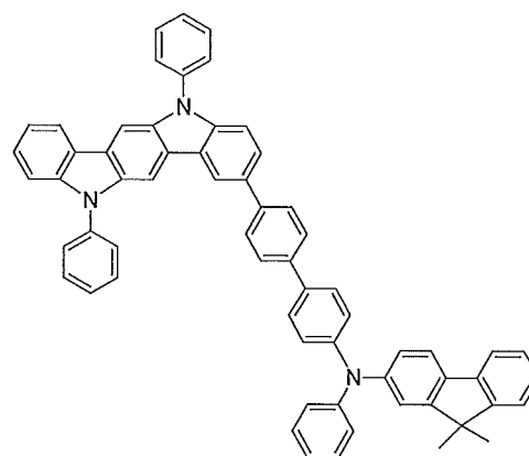
Compound 26
