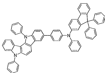
Compound 17
