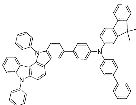
Compound 11
