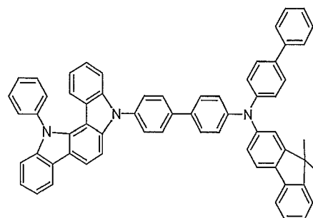
Compound 24
