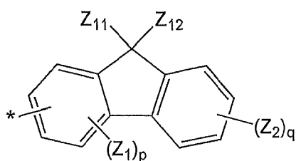
Formula 4D
