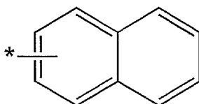
Formula 5B
