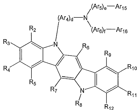
Formula 2d
