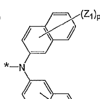
Formula 6C
