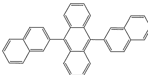
ADN
