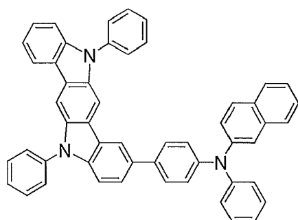
Compound 5
