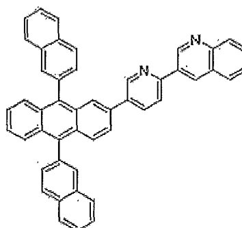
Compound 102
