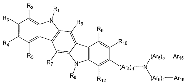
Formula 2b
