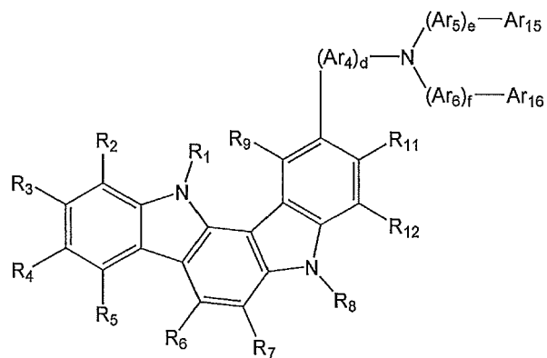
Formula 3a
