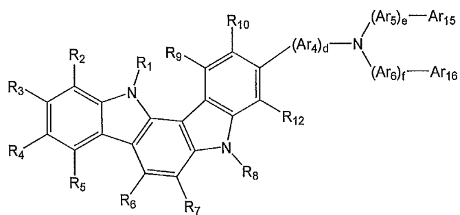
Formula 3b
