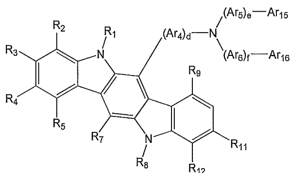
Formula 2c
