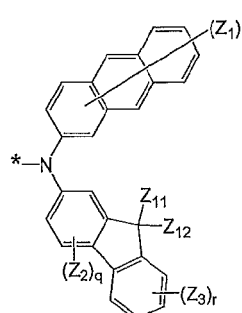
Formula 6I
