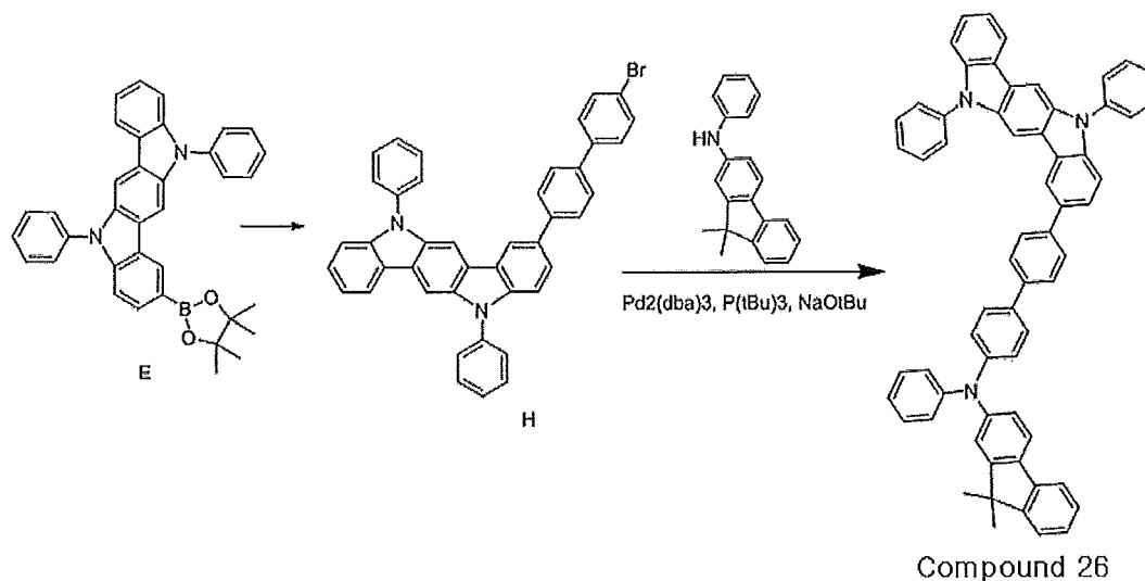
Reaction Scheme 5
