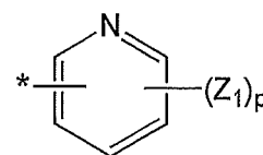
Formula 4F
