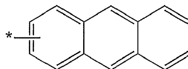
Formula 5C
