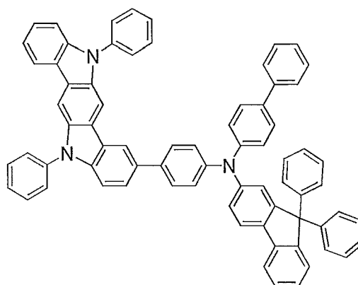
Compound 8
