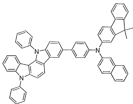
Compound 13
