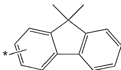
Formula 5D
