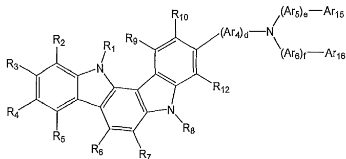
Formula 3b
