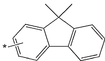
Formula 5D
