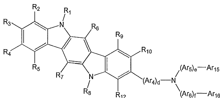
Formula 2b
