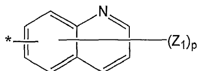
Formula 4G
