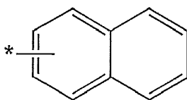
Formula 5B
