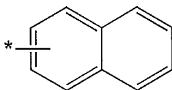
Formula 5B
