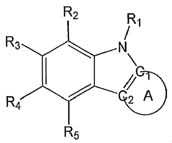
Formula 1
