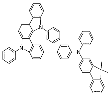
Compound 17
