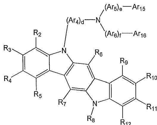
Formula 2d
