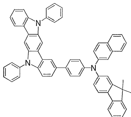
Compound 7
