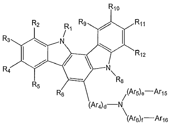
Formula 3d
