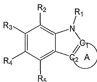
45 Formula 1
