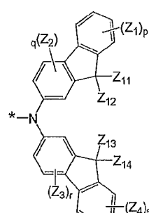
Formula 6K
