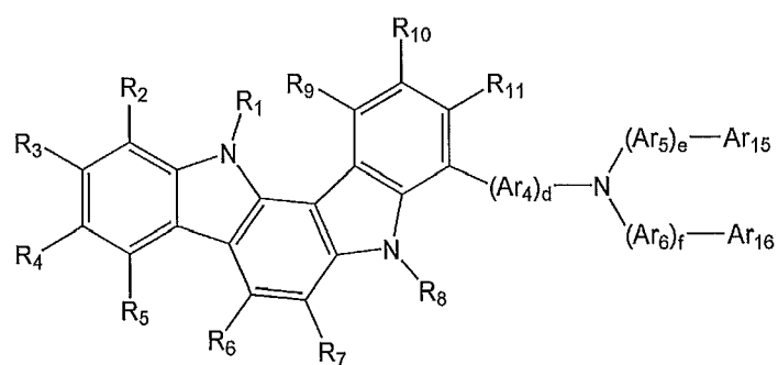
Formula 3c
