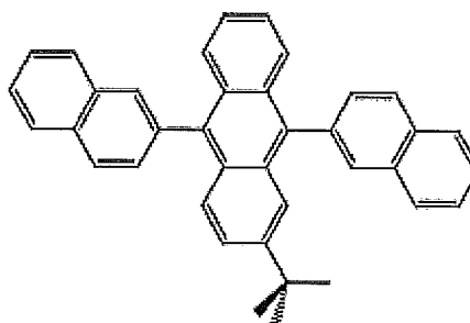
TBADN
