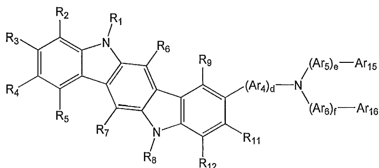
Formula 2a
