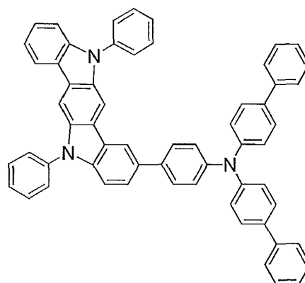
Compound 2
