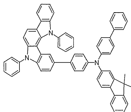
Compound 16
