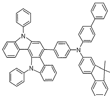
Compound 20
