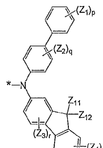
Formula 6J
