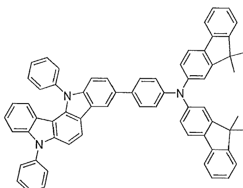
Compound 12
