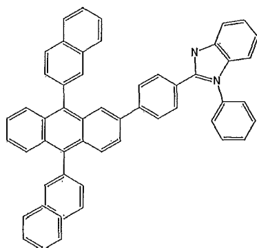
Compound 101
