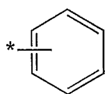
Formula 5A
