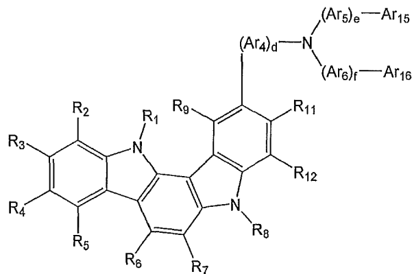
Formula 3a
