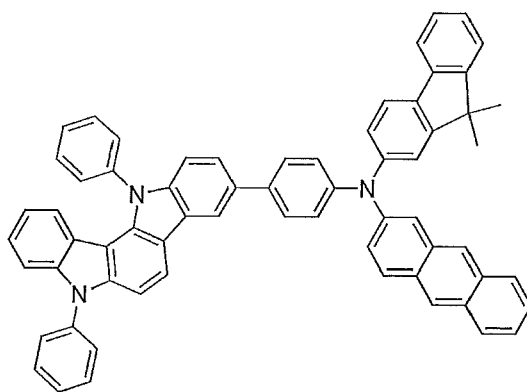
Compound 14
