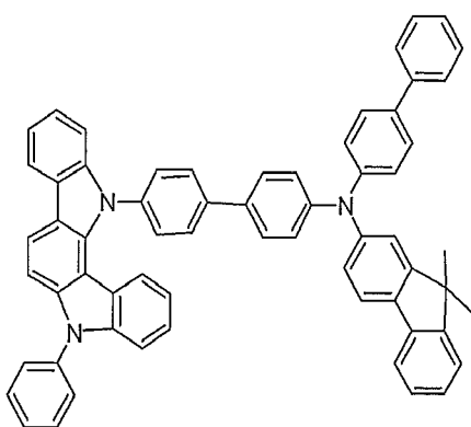
Compound 23
