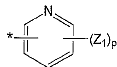
Formula 4F
