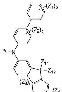
Formula 6J
