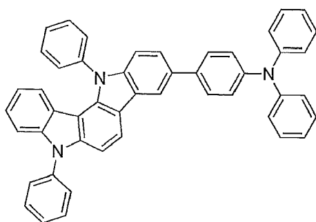
Compound 11
