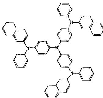
2T-NATA
