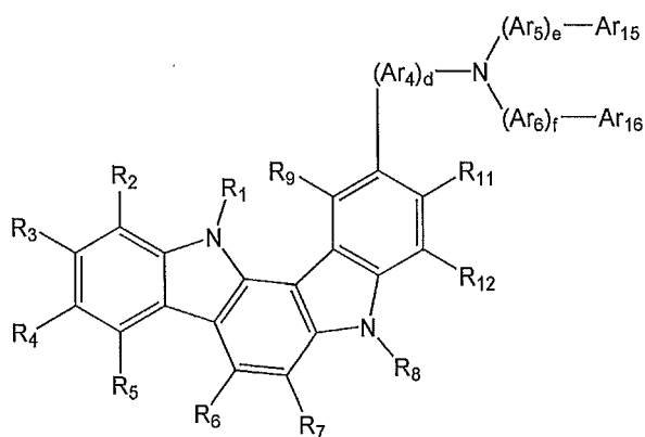
Formula 3a
