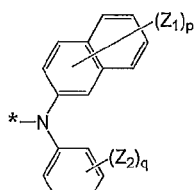
Formula 6B
