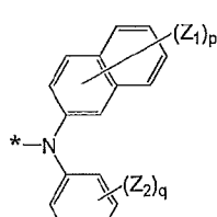
Formula 6B
