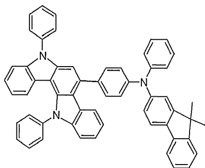
Compound 21
