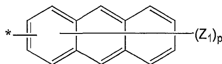
Formula 4C
