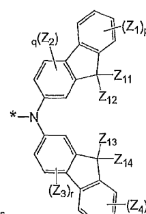
Formula 6K
