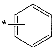
Formula 5A
