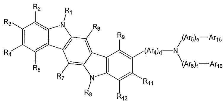
Formula 2a
