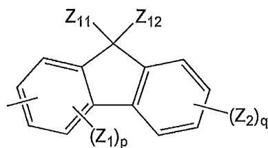
Formula 4D
