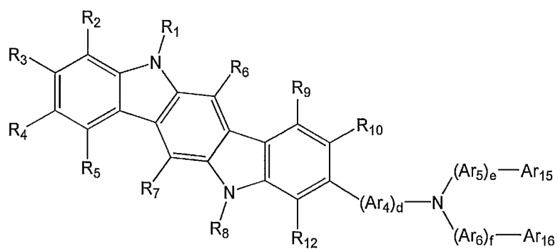
Formula 2b
