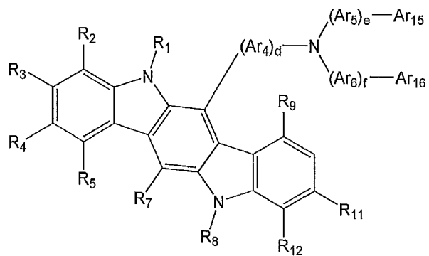
Formula 2c
