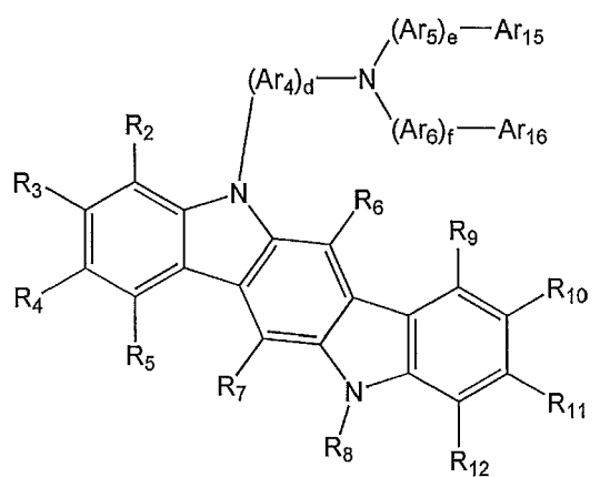
Formula 2d
