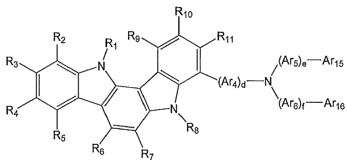
Formula 3c
