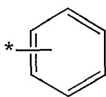
Formula 5A
