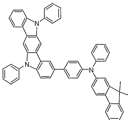
Compound 19
