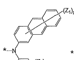
Formula 6D
