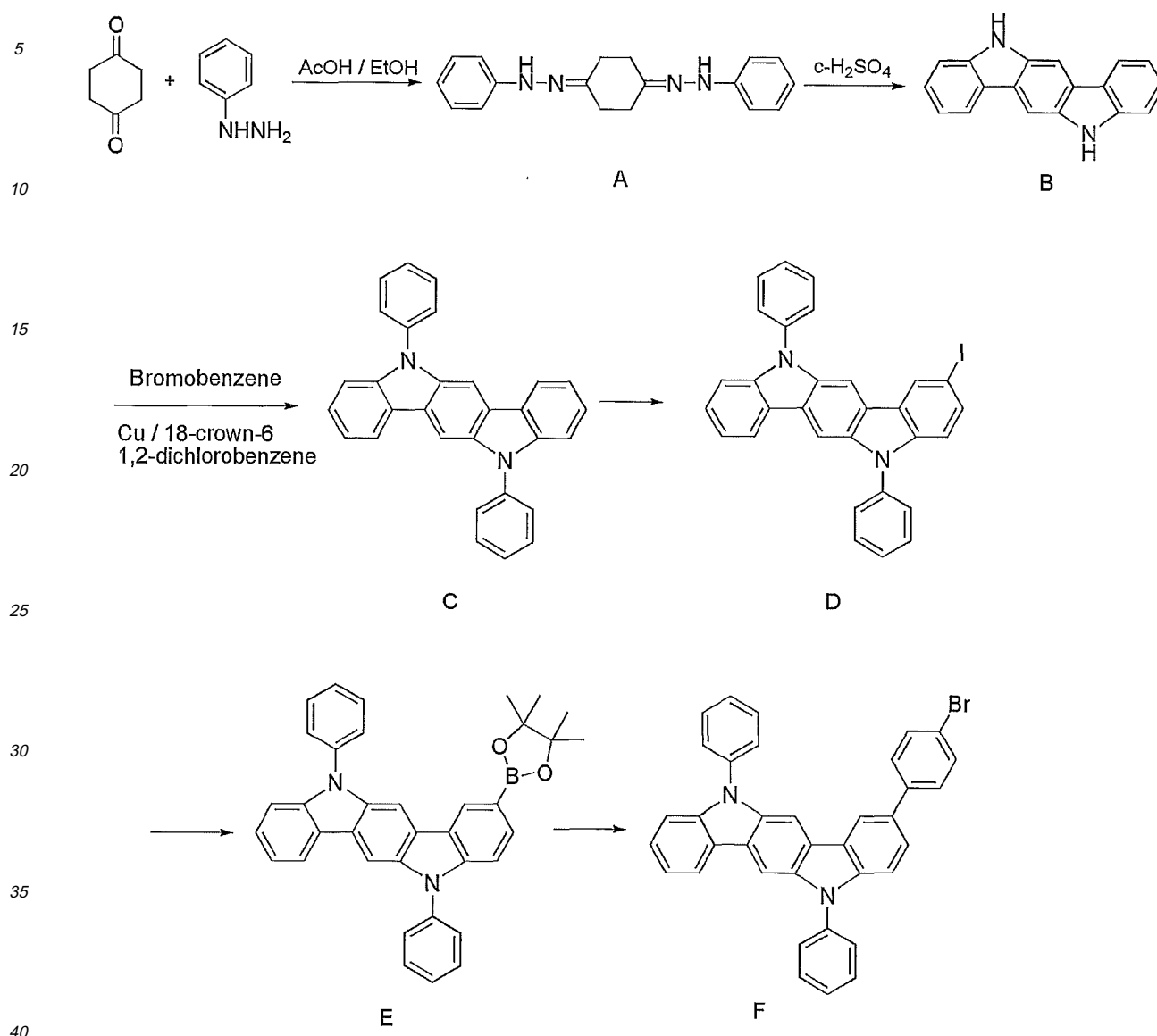
Reaction Scheme 1a
