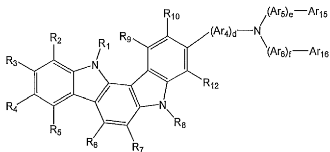
Formula 3b
