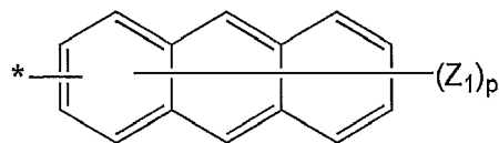
Formula 4C
