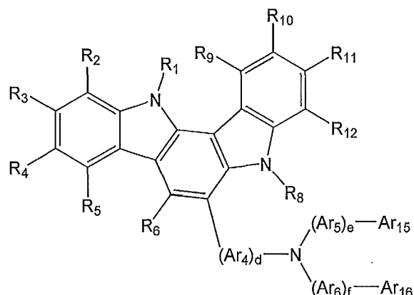
Formula 3d
