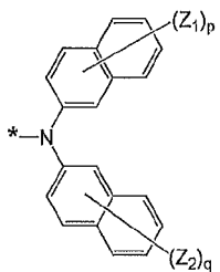
Formula 6C
