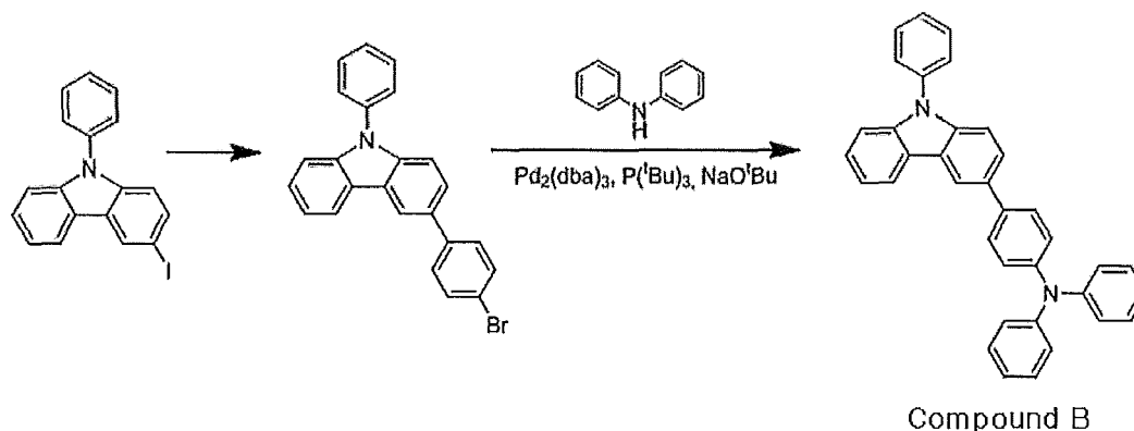
Reaction Scheme 8
