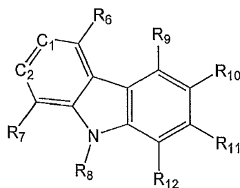
Formula 2
