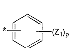
Formula 4A
