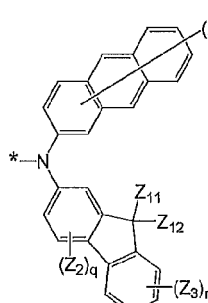
Formula 6I
