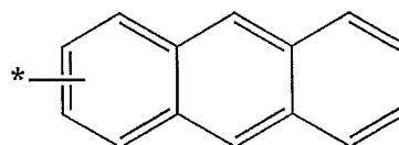
Formula 5C
