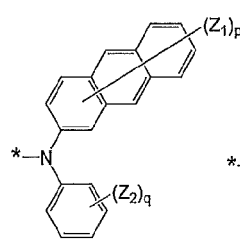
Formula 6D
