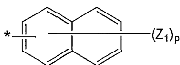
Formula 4B
