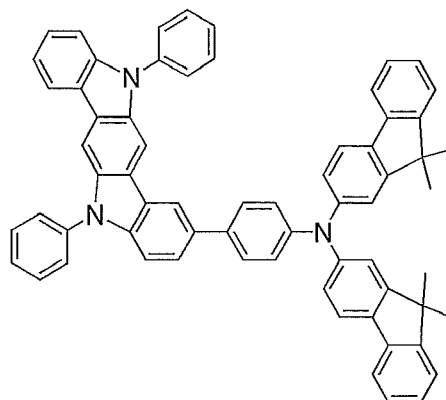
Compound 4
