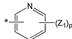
Formula 4F
