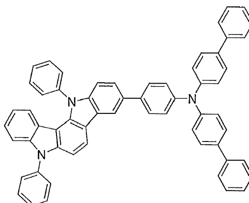
Compound 10
