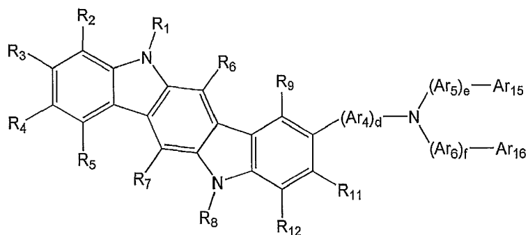
Formula 2a
