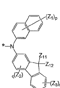
Formula 6H
