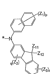
Formula 6H
