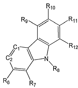
Formula 3
