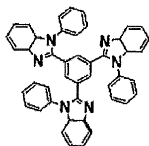
TPBI
