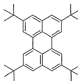
TBP
