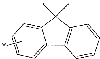
Formula 5D
