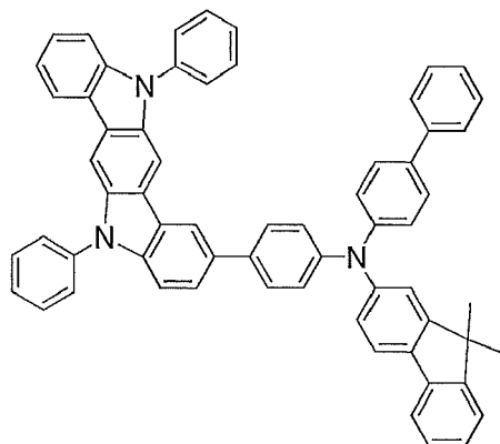
Compound 3
