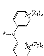
Formula 6A
