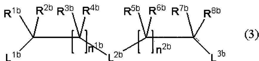
Chemical Formula 8
