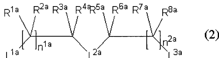
Chemical Formula 4
