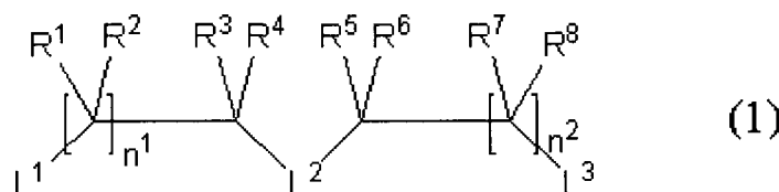
Chemical Formula 1
