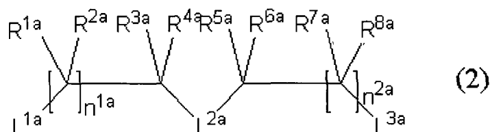
Chemical Formula 4
