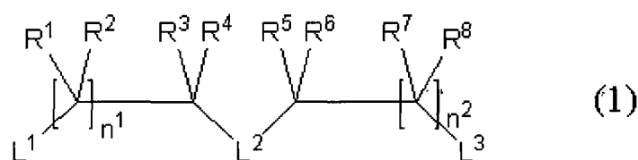
Chemical Formula 6
