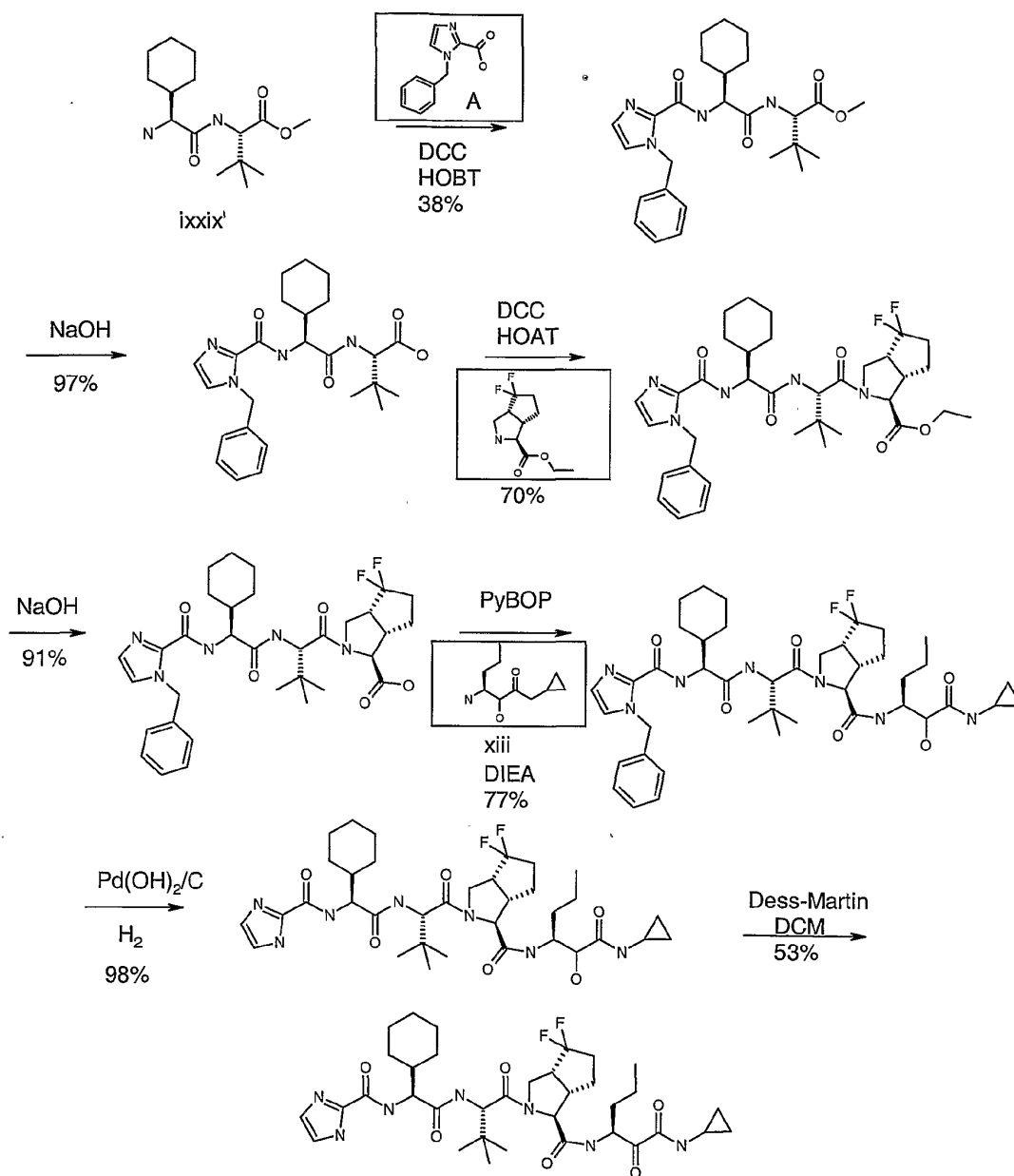
Scheme 11
