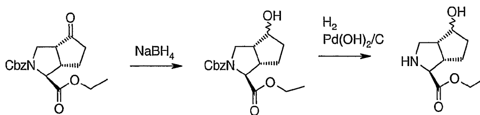
SCHEME 6
