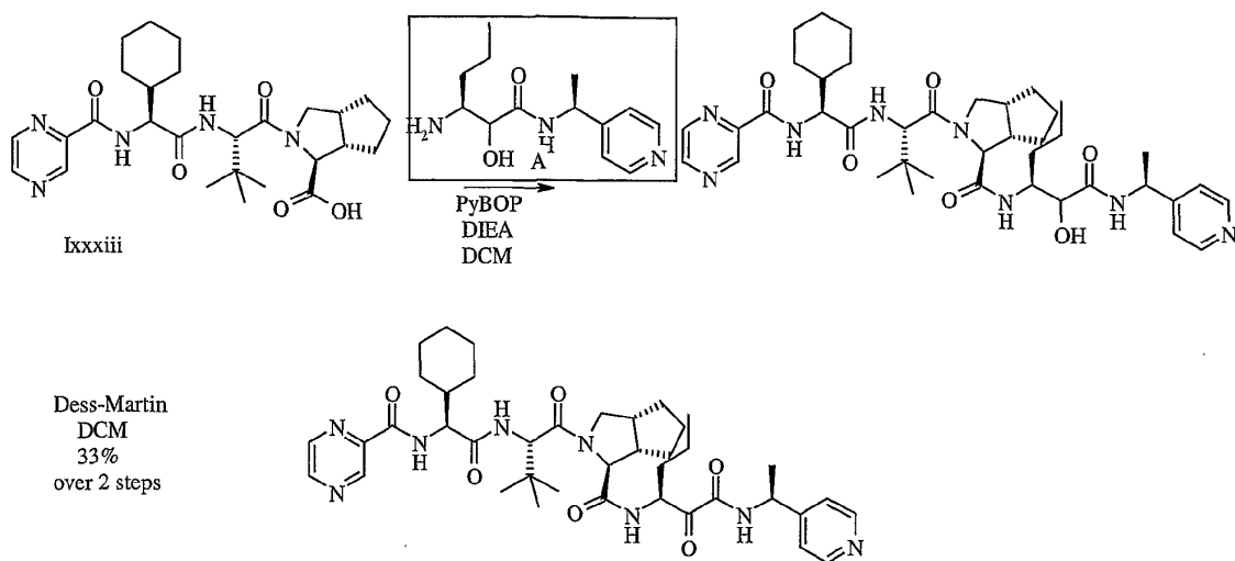
Scheme 9
