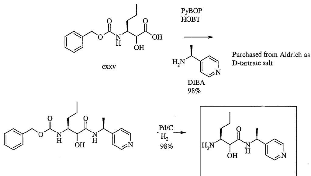
SCHEME 10
