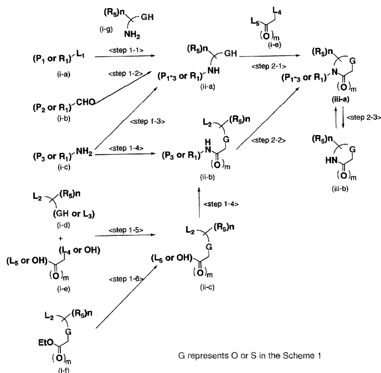
Scheme 1 Synthetic route of the key intermediate (iii-a)
