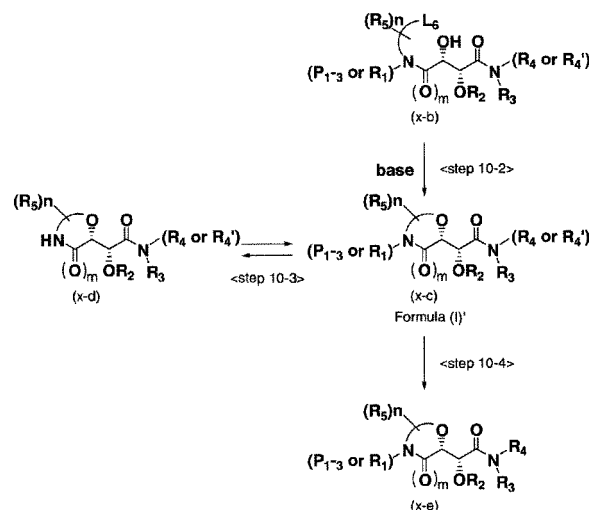
Scheme 6 Synthetic route of optically active compounds (x-c) and (x-e)
