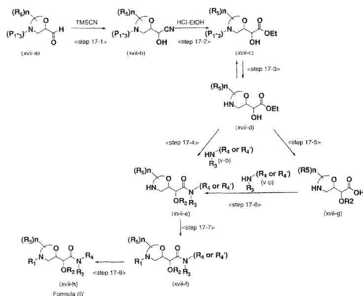
Scheme 15 Alternative synthetic route of morpholine compounds.
