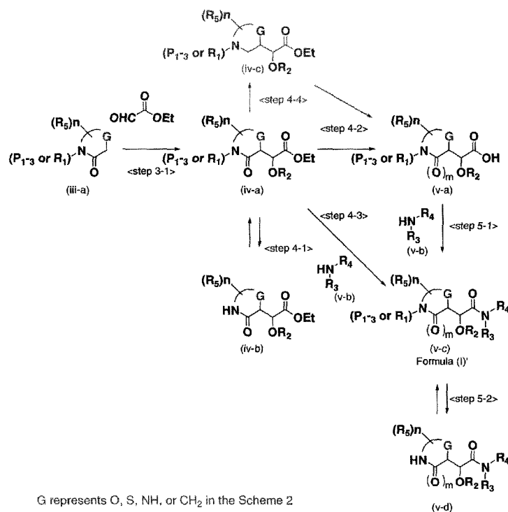
Scheme 2 Synthetic route of Example compounds and combination compounds.
