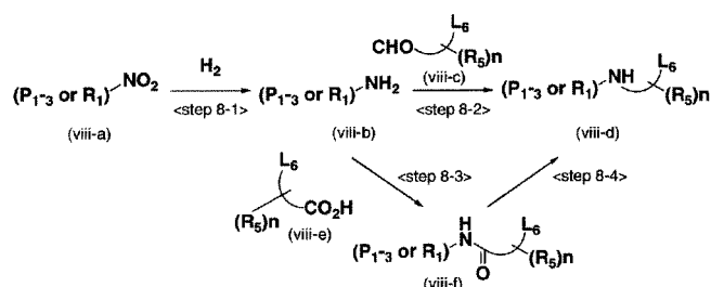
Scheme 4 Synthetic route of intermediate compounds (viii-d)
