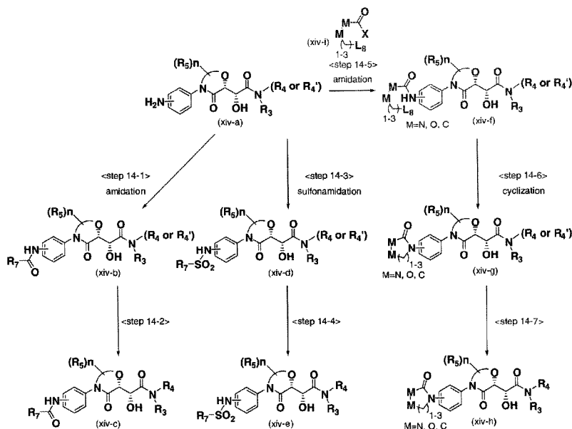
Scheme 12 Synthetic route of R1 aniline derivative compounds (xiv-b), (xiv-c), and (xiv-d) from aniline analogue compound represented by formula (xiv-a)
