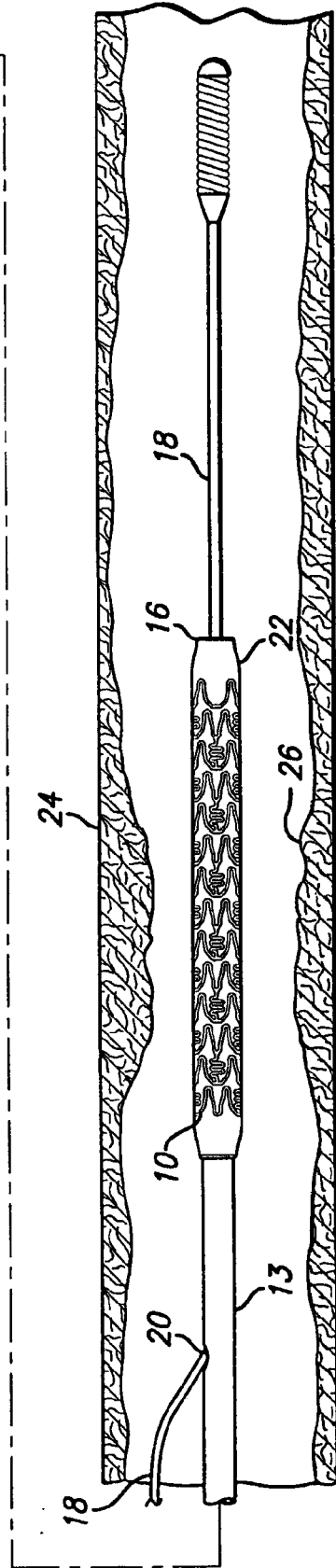
FIG. 2 PRIOR ART
