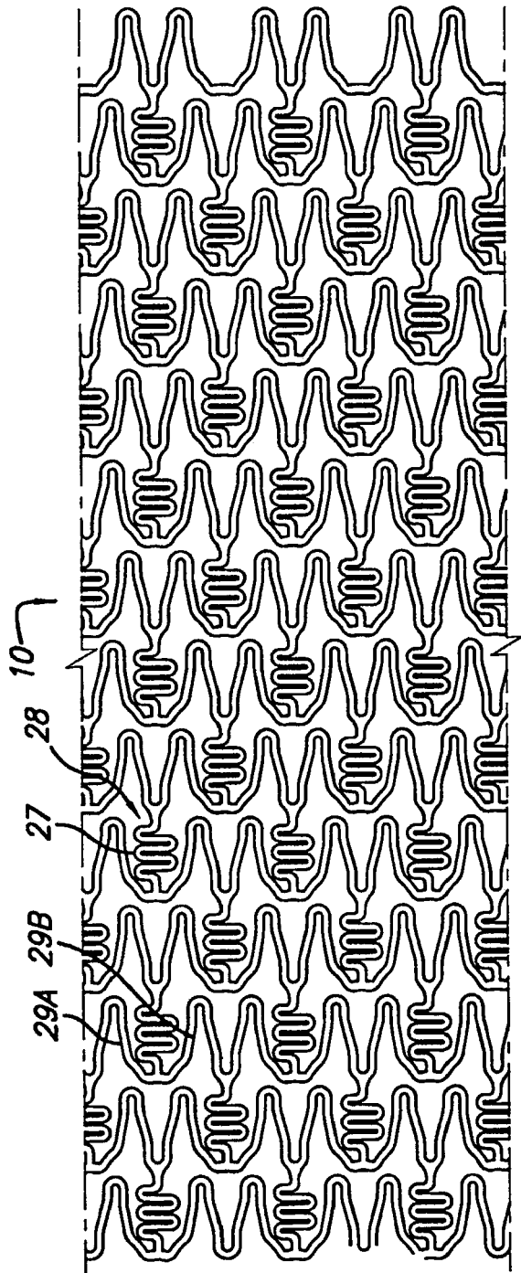
FIG. 4 PRIOR ART
