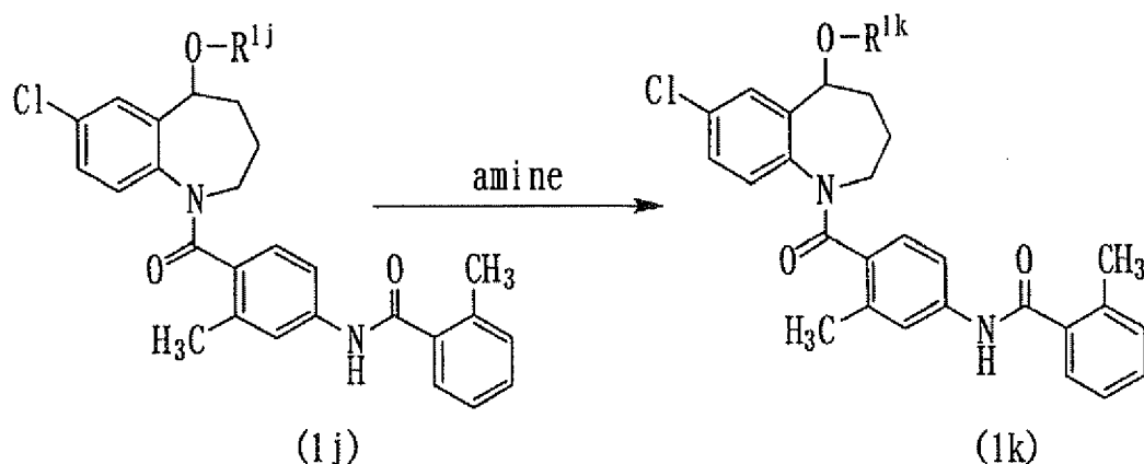
Reaction Scheme-10
