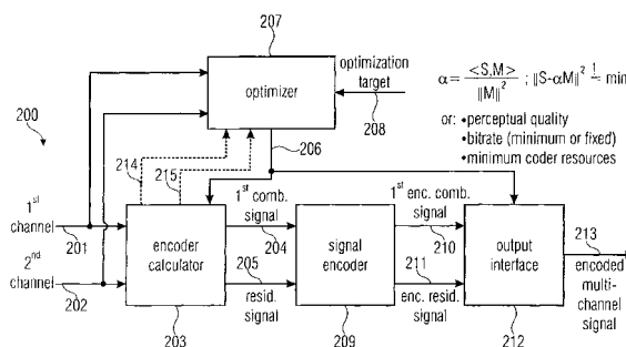
FIGURE 2 (AUDIO ENCODER)
