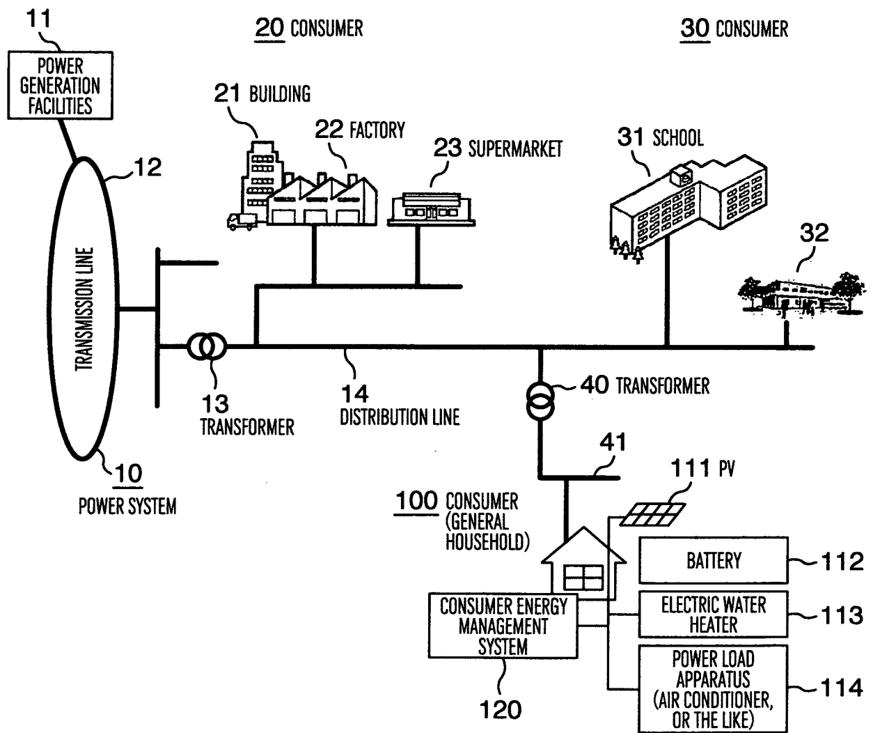
SYSTEM CONFIGURATION EXAMPLE OF FIRST EMBODIMENT
