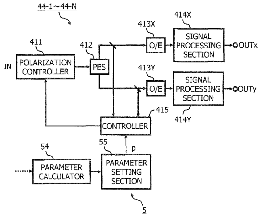
OPTICAL RECEIVER CONFIGURATION EXAMPLE (2)
