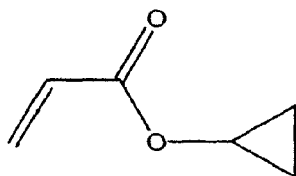
methylene cyclopropyl acetic acid
