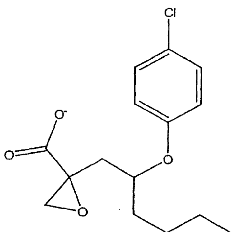
2-[b-(4-chlorophenoxy)-hexyl]oxirane-2-carboxylate
