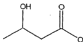
3-hydroxybutyrate beta-hydroxybutyrate
