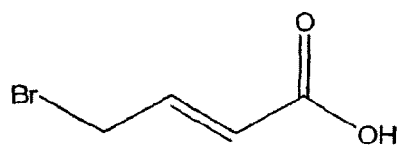
4-bromocrotonic acid
