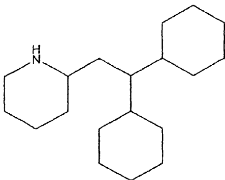
perhexiline
