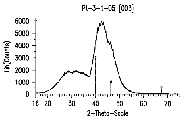
Pt-3-1-05 [003] Pt-3-1-05 [003] - File: Pt-3-1-05_01 [003].raw - Type: 2Th alone - Start: 15.000° - End: 75.000° - Step: 0.050° - Step time: 3599.8 s - Temp.: 25°C (Roo Operations: Range Op. Merge | Import [003] 01-1194 (D) - Platinum - Pt - Y: 50.00 % - d x by: 1. - WL: 1.54056 - Cubic - a 3.91610 - b 3.91610 - c 3.91610 - alpha 90.000 - beta 90.000 - gamma 90.0
