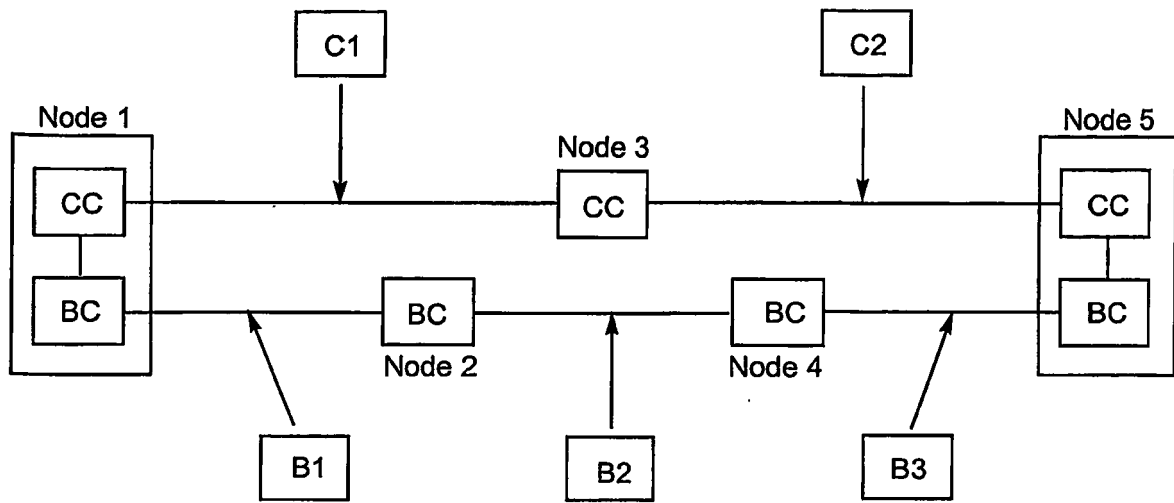
Figure 2 (Prior Art)
