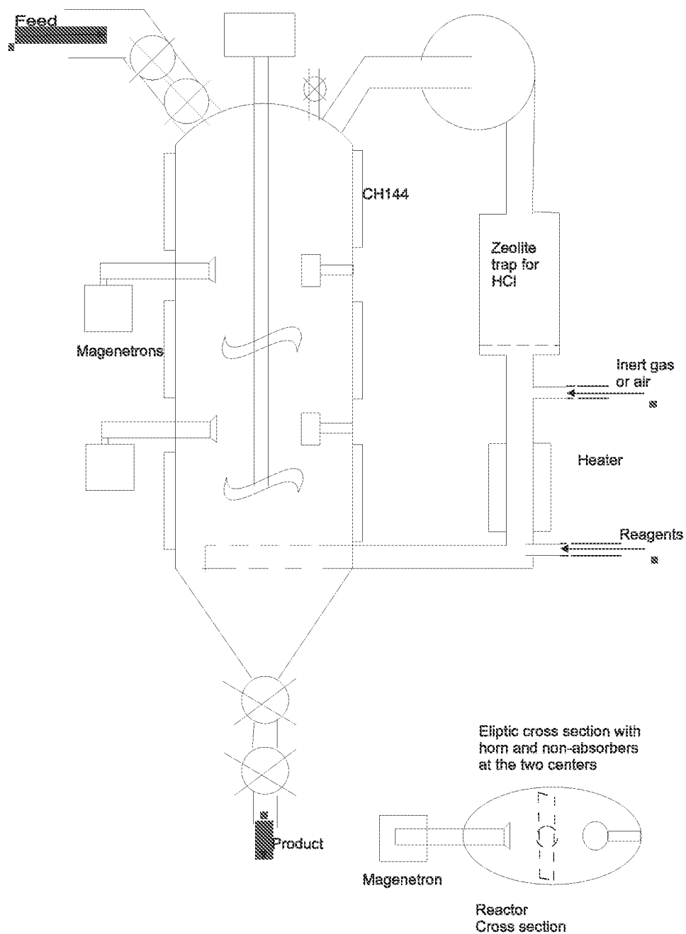
Fig. 7 Microwave assisted grafting
