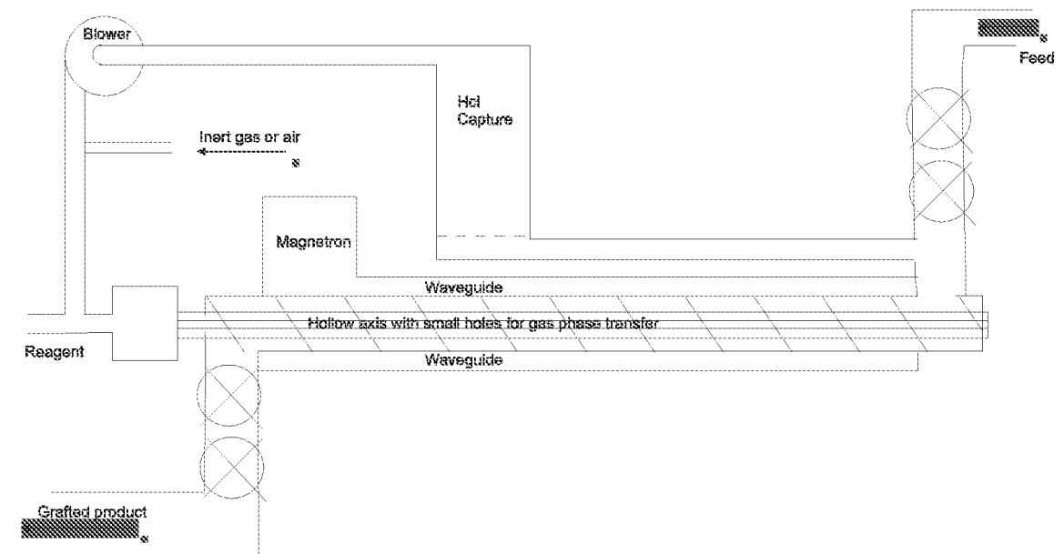
Fig. 8 Equipment for continuous microwave assisted grafting of fibres
