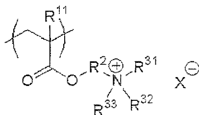
Formula (VI)
