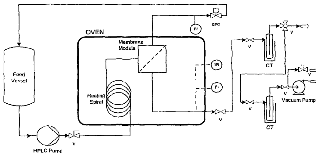
Figure 1- Schematic drawing of the pervaporation set up (V: valve, PI: pressure indicator, TR: temperature recorder, BPC: back pressure controller, CT: cold trap)
