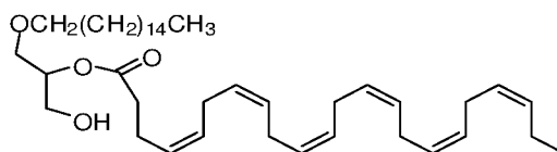
(4Z,7Z,10Z,13Z,16Z,19Z)-1-(hexadecyloxy)-3-hydroxypropan-2-yl docosa-4,7,10,13,16,19-hexaenoate
