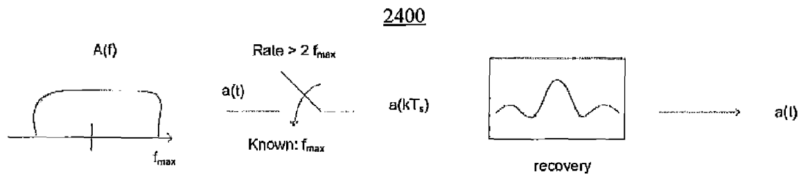
FIG. 24 PRIOR ART
