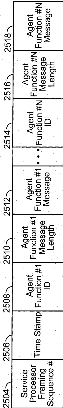
Service Processor Communication Frame 2502
