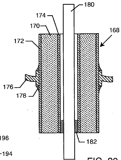
FIG. 30 PRIOR ART
