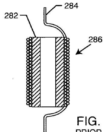
FIG. 56 PRIOR ART
