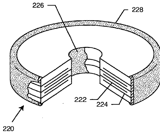
FIG. 39 PRIOR ART
