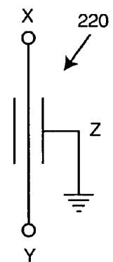
FIG. 41 PRIOR ART
