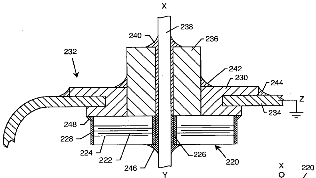
FIG. 40 PRIOR ART
