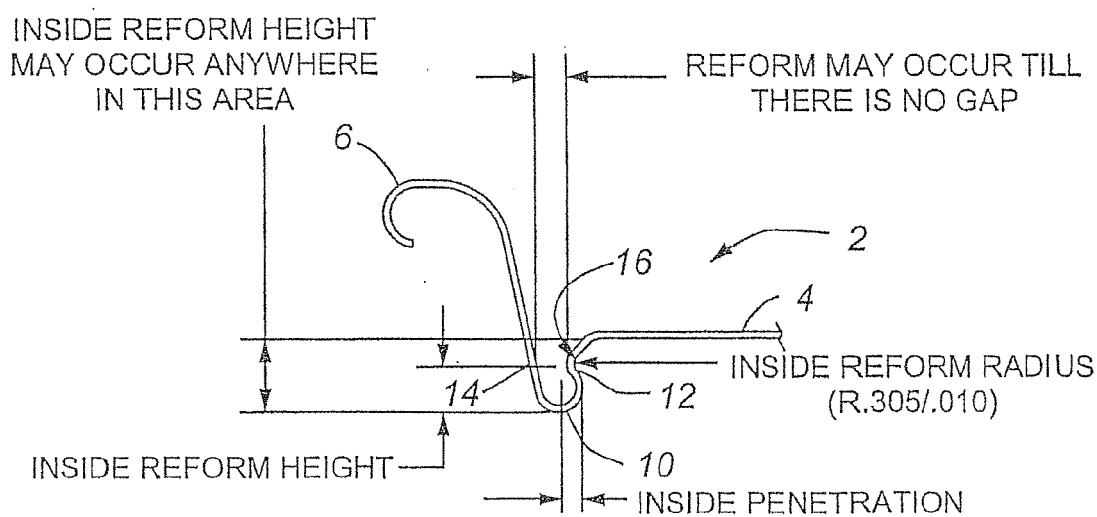
INSIDE REFORMING
