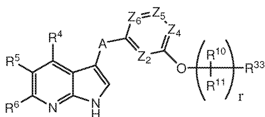
Formula IIId
