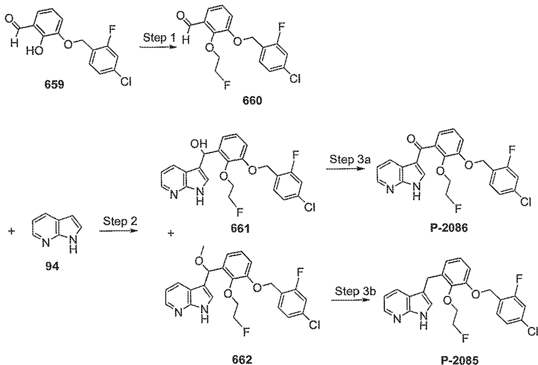
Scheme 82
