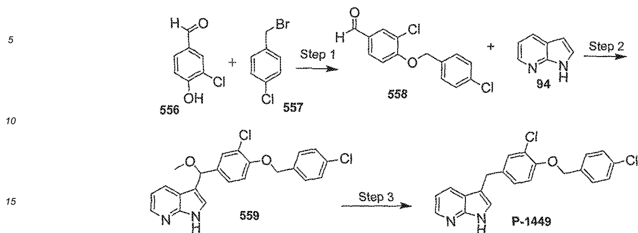
Scheme 51
