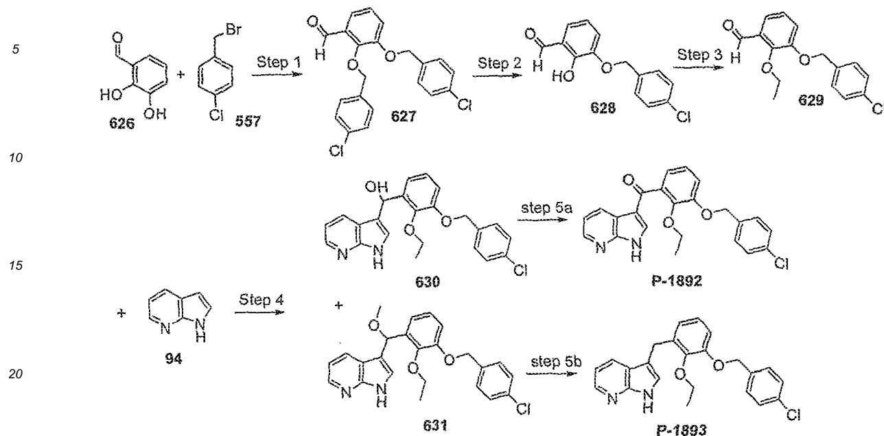
Scheme 71
