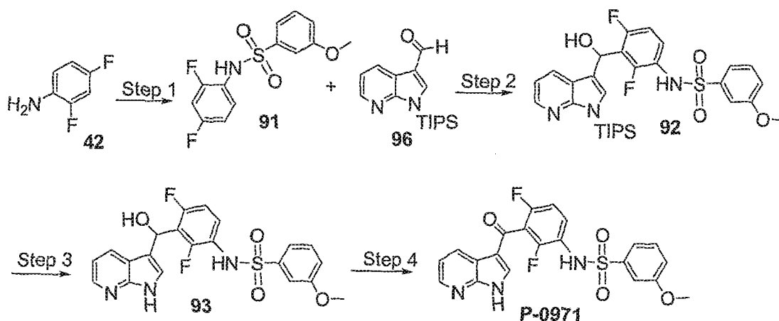
Scheme 26
