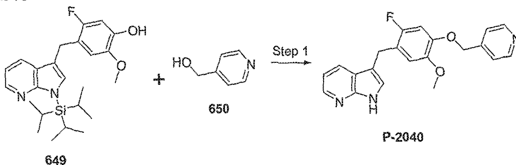
Scheme 78
