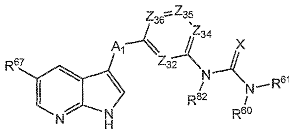
Formula IIIg
