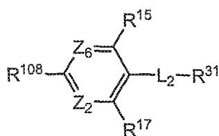
Formula IV
