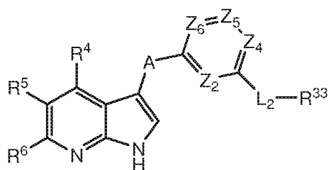
Formula IIIo
