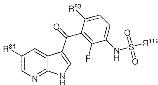
Formula IIIIm
