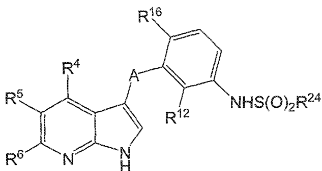
Formula IIa
