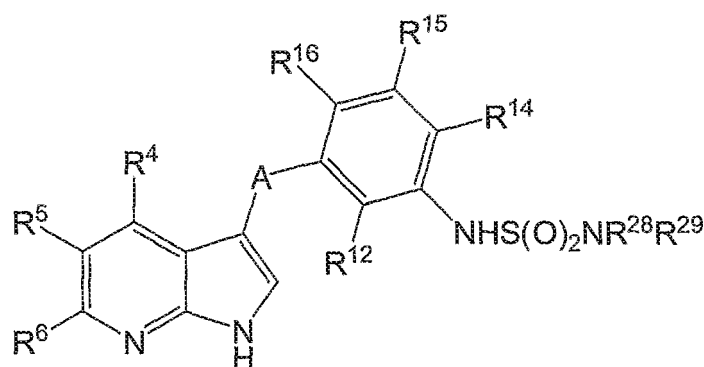
Formula IIb
