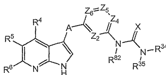
Formula IIIf
