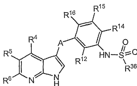
Formula IIIj
