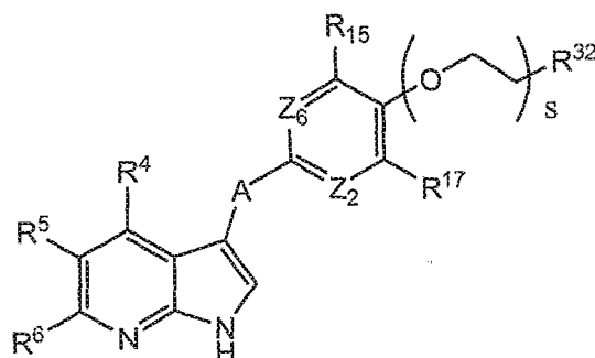
Formula IIIc
