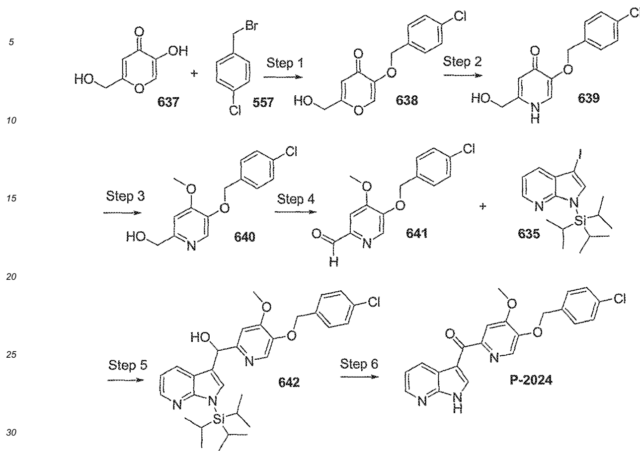
Scheme 75
