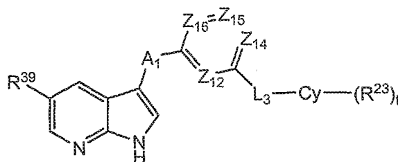
Formula IIIq
