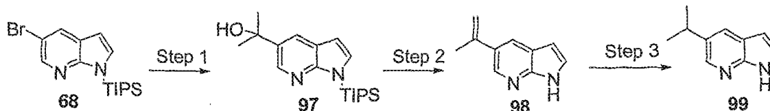
Scheme 28
