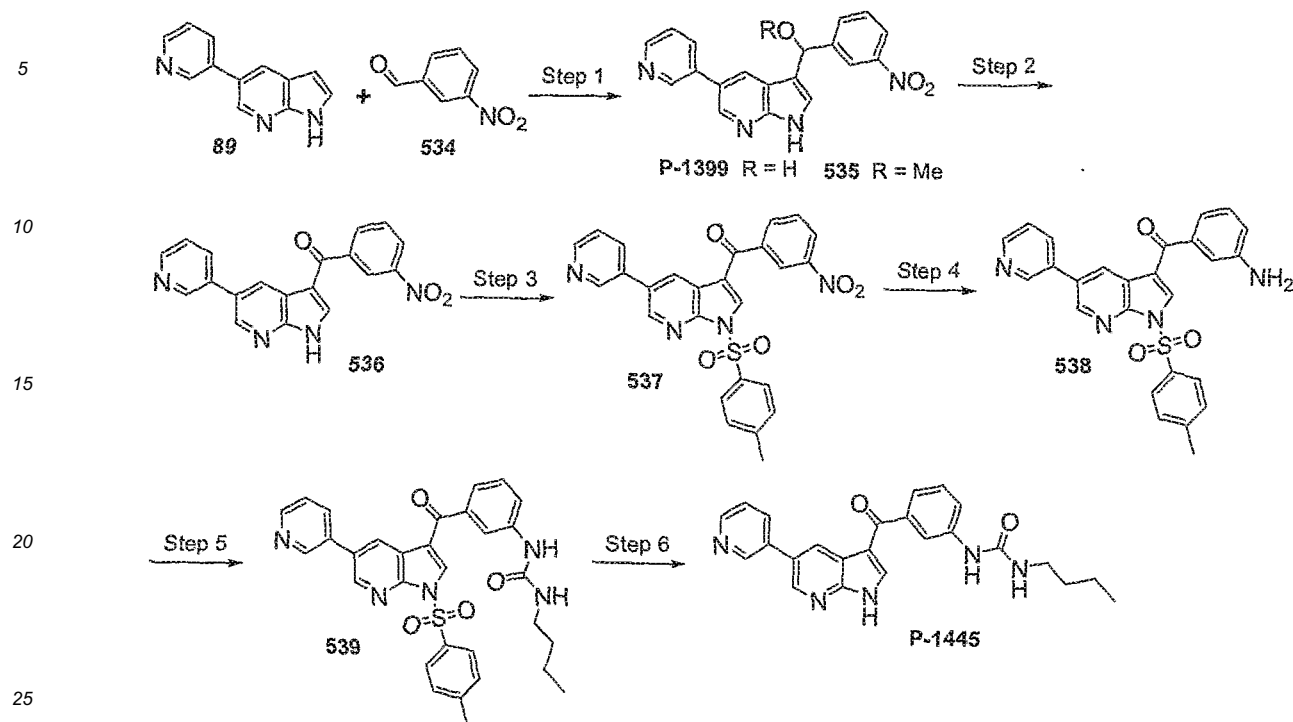
Scheme 49
