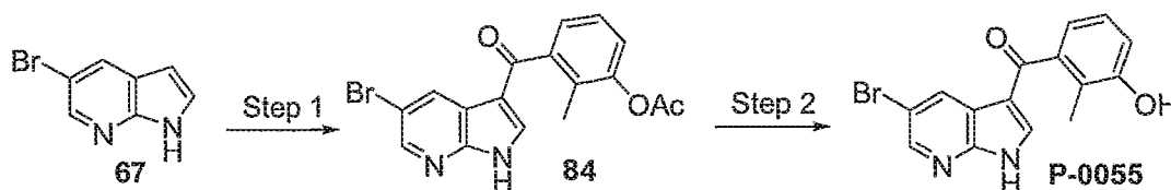
Scheme 22
