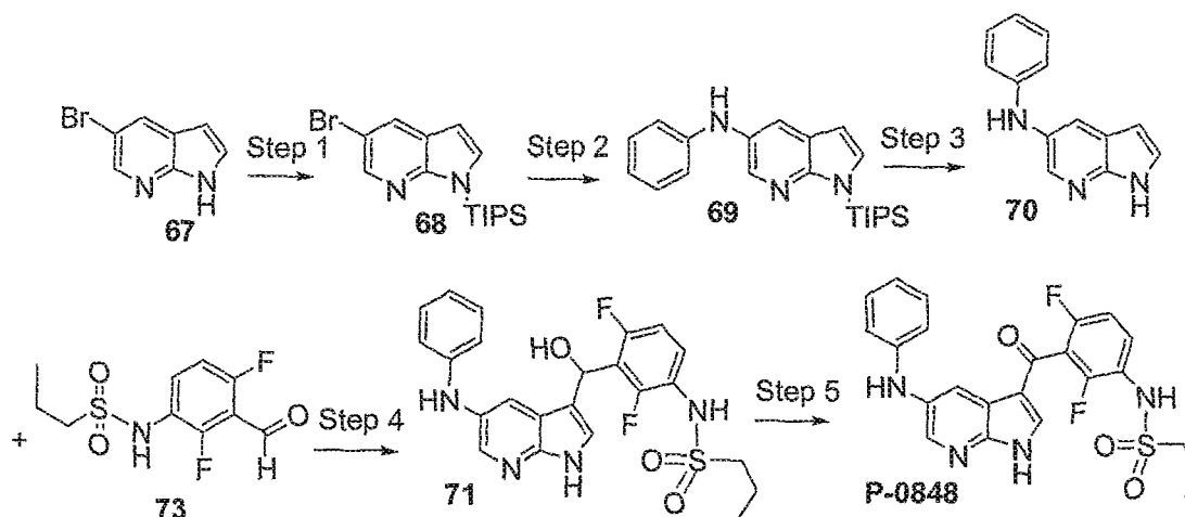
Scheme 18
