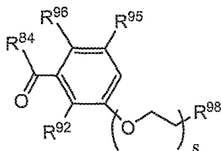
Formula IXa
