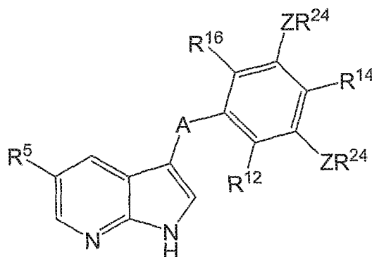
Formula IIo
