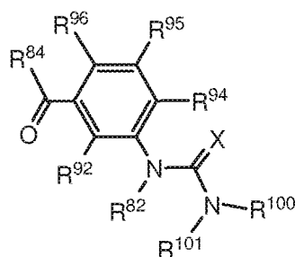
Formula VIIIb
