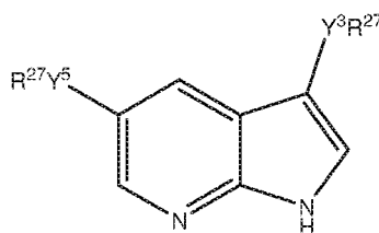
Formula Ia
