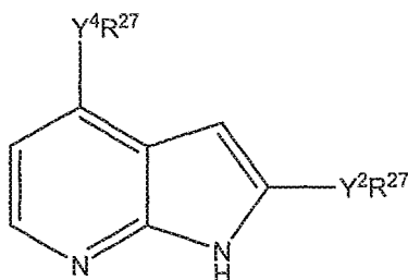
Formula Ie
