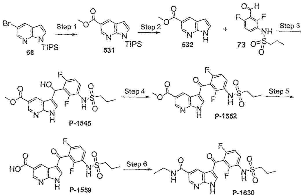
Scheme 45
