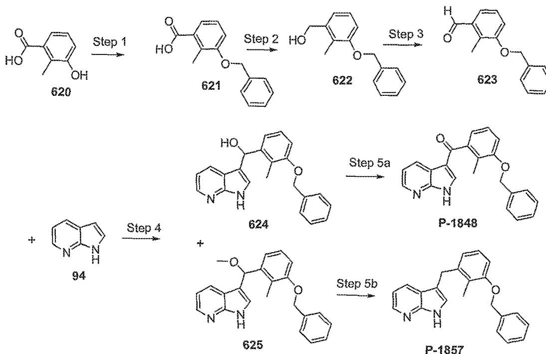
Scheme 70
