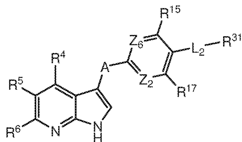
Formula IIIa
