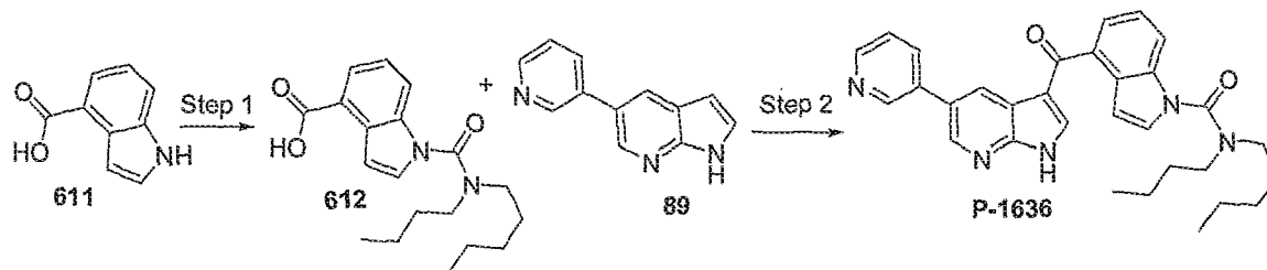
Scheme 68
