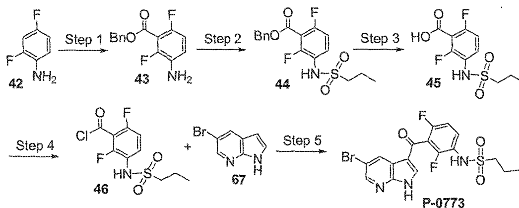
Scheme 13
