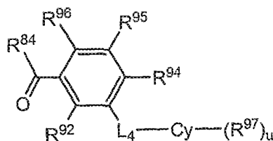
Formula VIa
