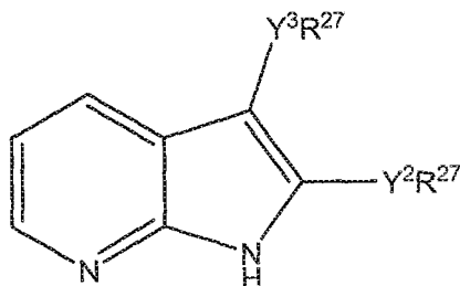
Formula Id
