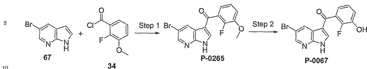
Scheme 10
