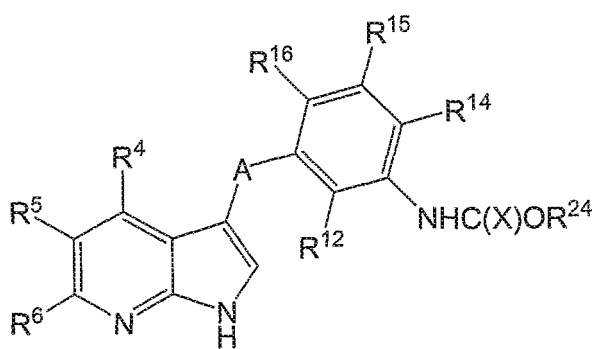
Formula IIe
