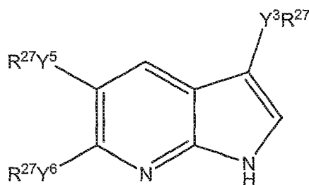
Formula Iy
