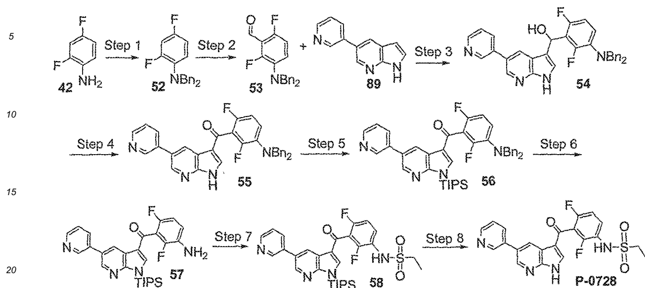
Scheme 16
