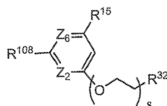
Formula IX
