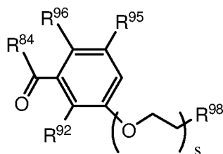
Formula IXa
