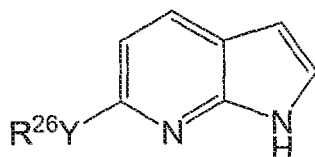
Formula In
