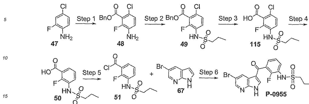
Scheme 14
