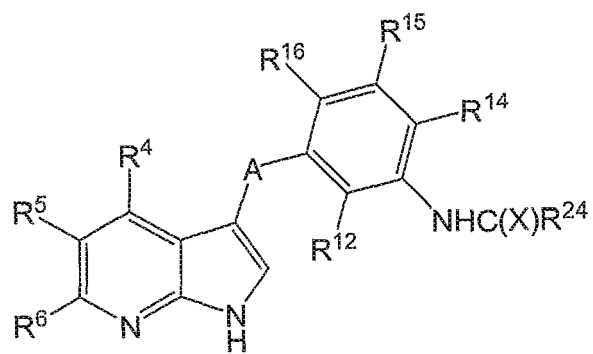
Formula IIc
