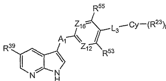
Formula IIIb
