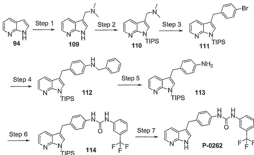
Scheme 34
