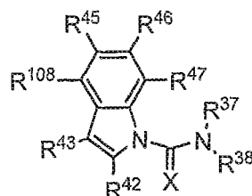
Formula VIII
