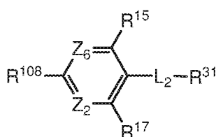
Formula IV
