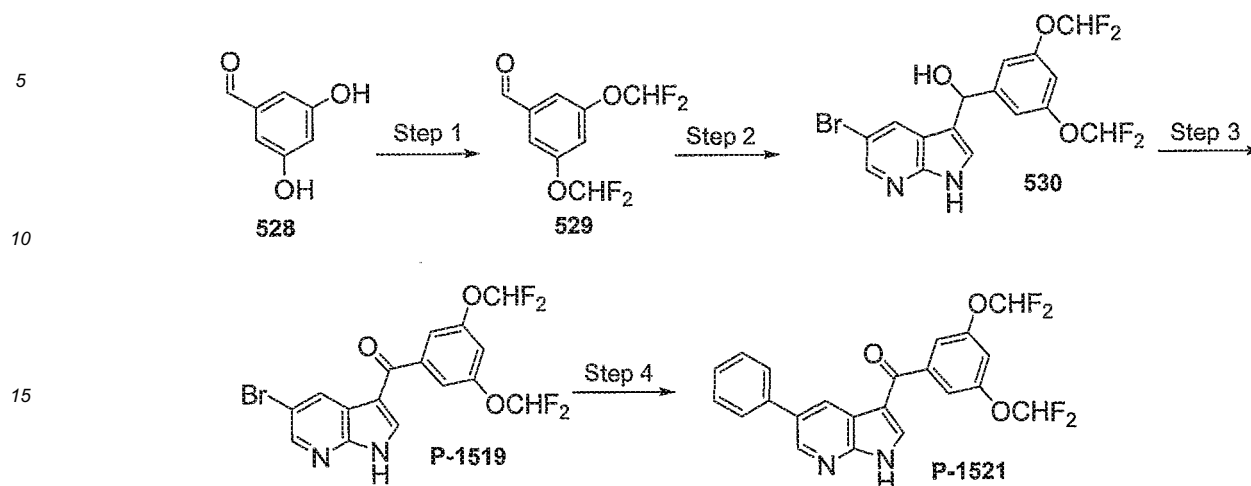
Scheme 44
