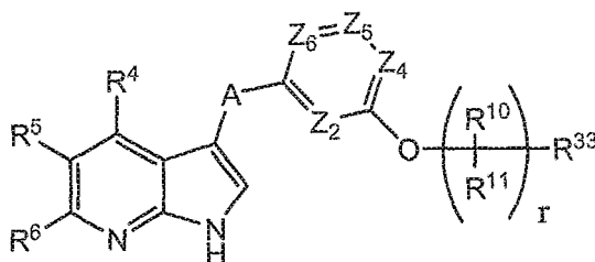
Formula IIIId
