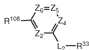
Formula VI
