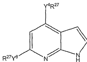
Formula Ih
