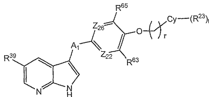
Formula IIIp
