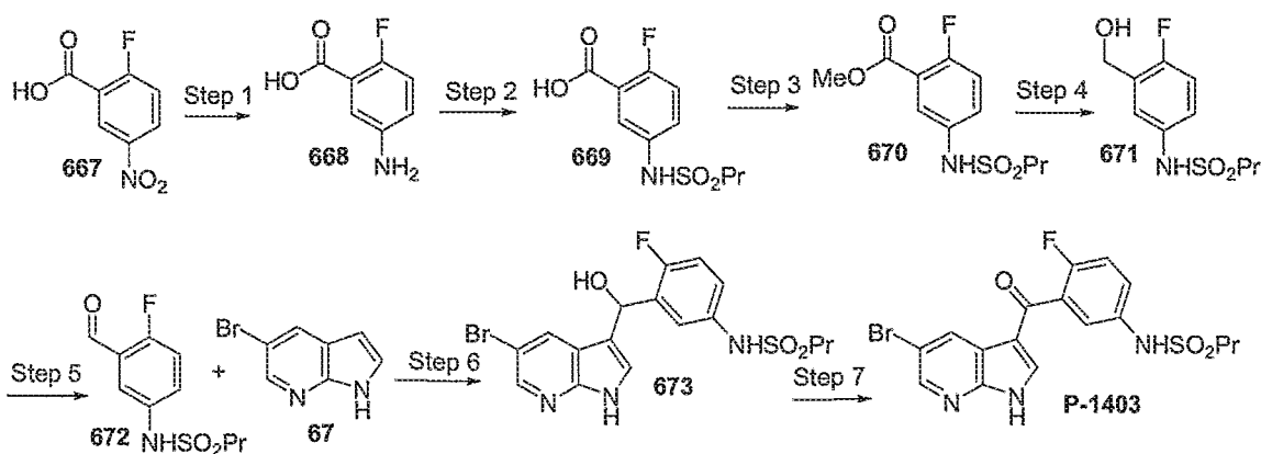
Scheme 84
