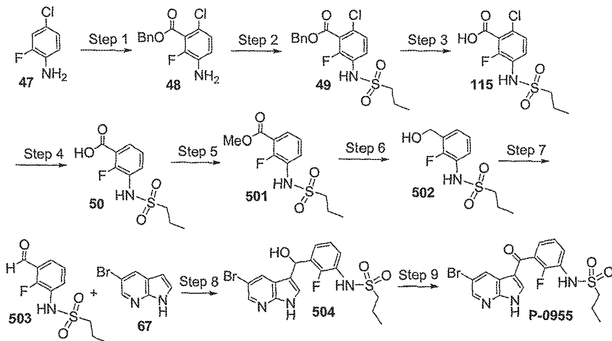
Scheme 37
