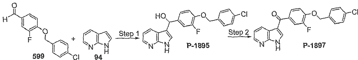
Scheme 63
