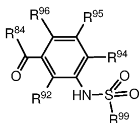
Formula VIIa
