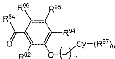
Formula VIb
