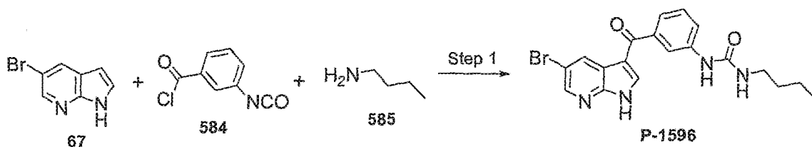
Scheme 55
