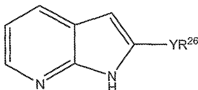
Formula Ip
