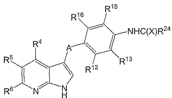
Formula IIIi
