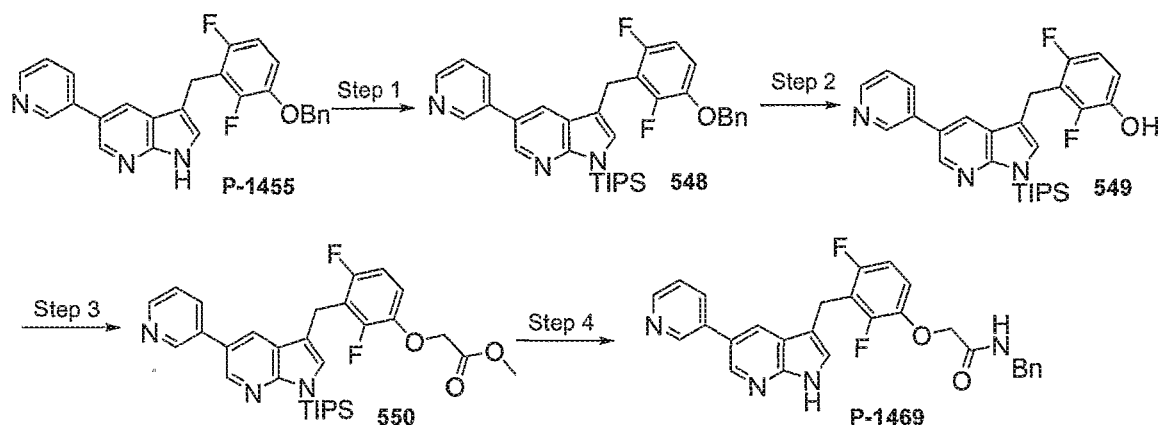
Scheme 46
