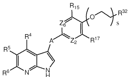
Formula IIIc
