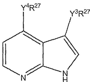
Formula Ib
