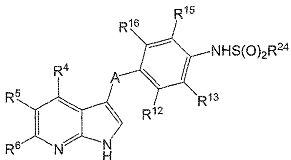
Formula IIIk
