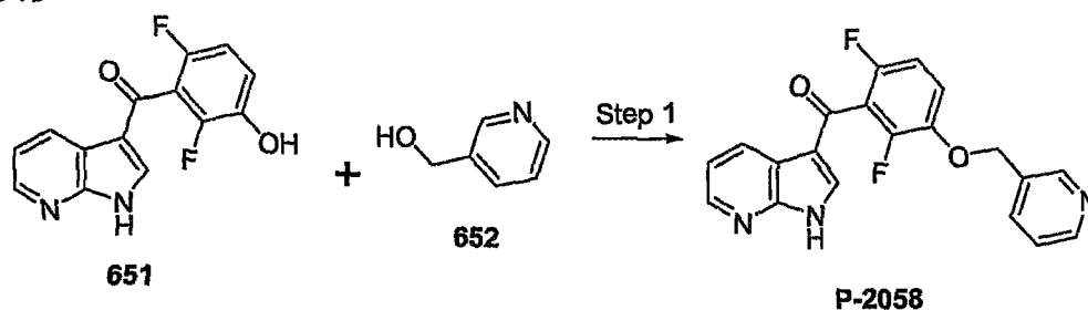
Scheme 79
