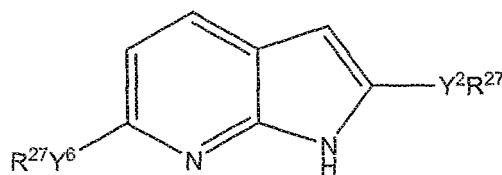
Formula Ig
