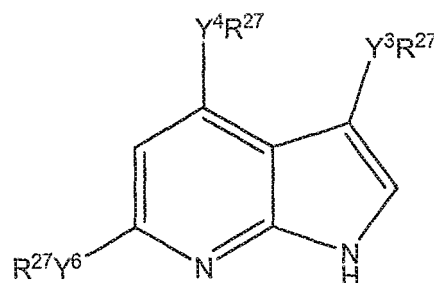
Formula Ix
