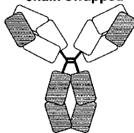
III. VH and L chain swapped
