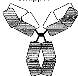
I. Fd and L chain swapped
