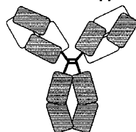
IV. CH1 and CL chain swapped
