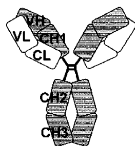
I. Fd and L chain swapped
