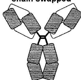
II. VH and VL chain swapped
