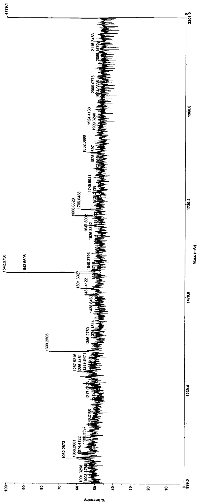
Voyager Spec #1[BP = 1542.6, 4779]
