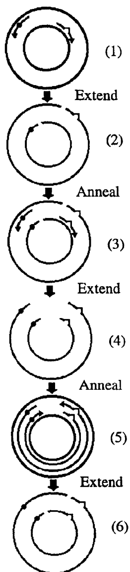
Figure 12 Site-Directed Mutagenesis by Polymerase-based Extension
