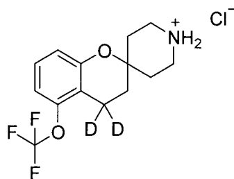
5-(Trifluoromethoxy)-3,4-dihydrospiro[chromene-2,4'-piperidinium] chloride- d_2
