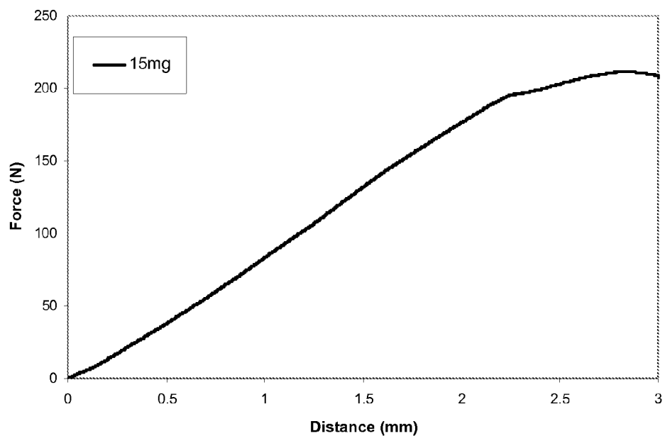
Example 20 Indentation Test of Example 14.2 tablet
