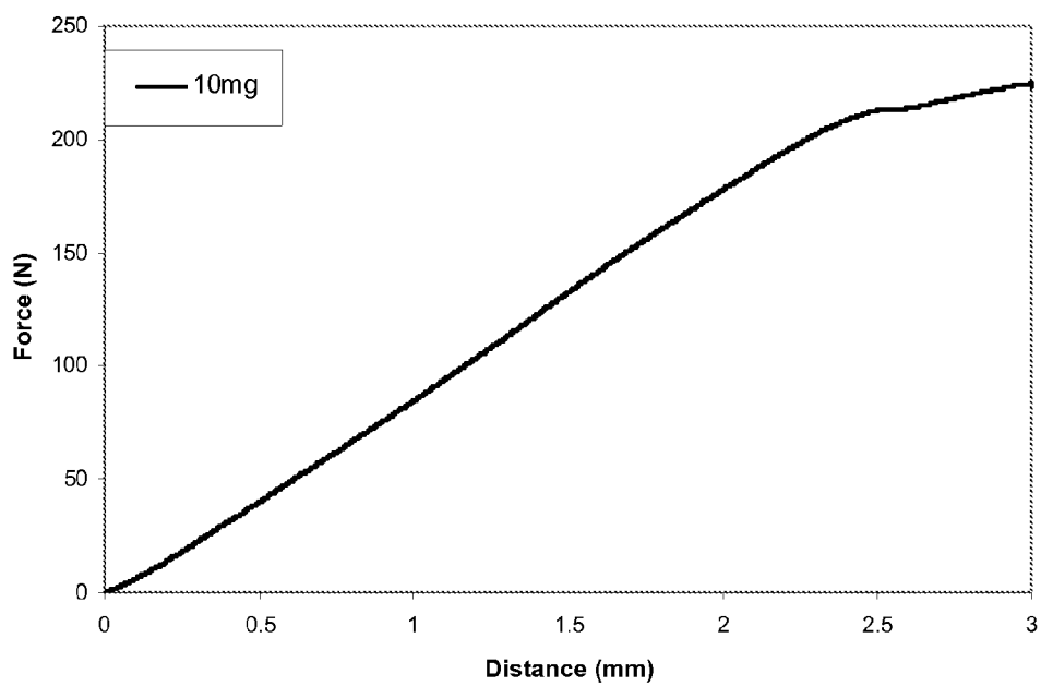
Example 20 Indentation Test of Example 14.1 tablet
