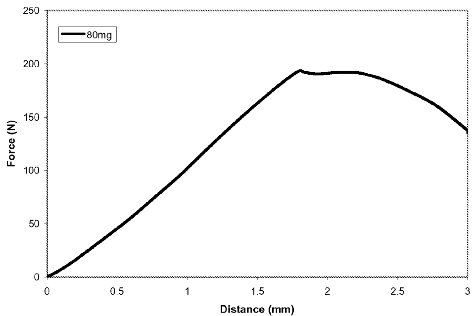
Example 20 Indentation Test of Example 18.2 tablet
