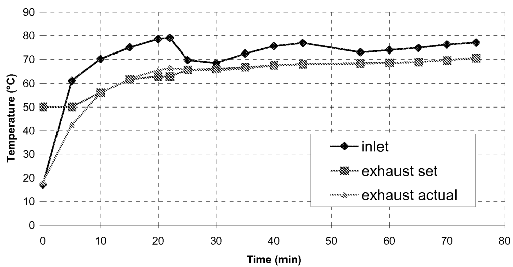
Curing of Example 14.3 Temperature Profile
