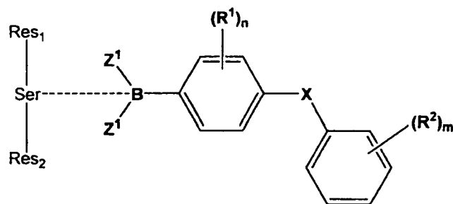
(III-b)-complex
