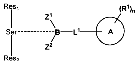
(II)-complex
