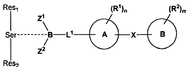
(III)-complex
