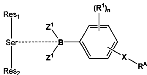
(III-a)-complex
