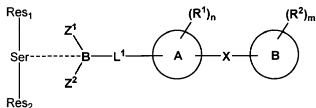
(III)-complex
