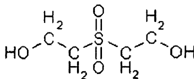
bis(2-hydroxyethyl) sulfone
