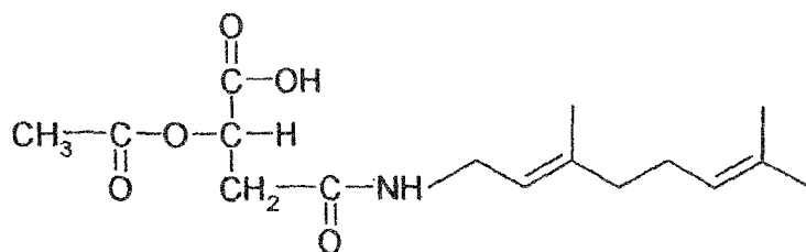
O-acetyl-N,N'-digeranylmalic diamide
