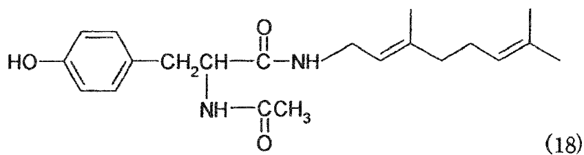
N-acetyltyrosine geranylamine
