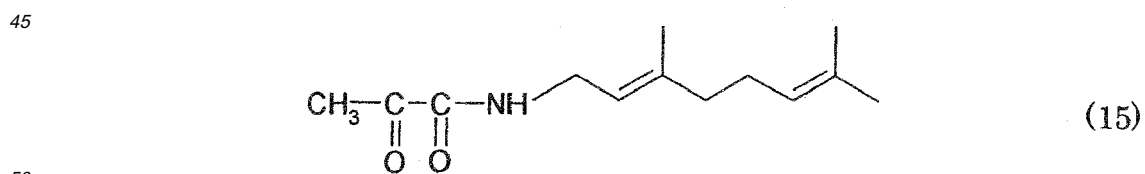
N-geranyl-p-pyruvoaminobenzamide
