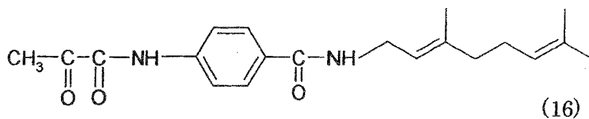
tyrosine geranylamine
