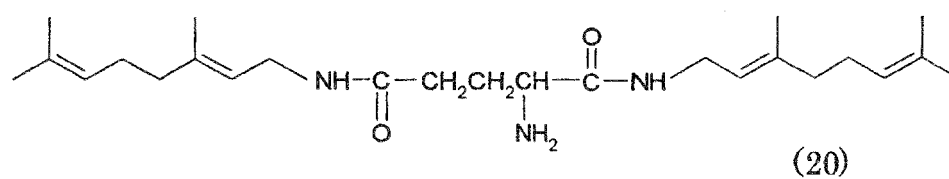
serine geranylamine
