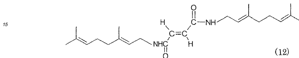
N-geranylfumaric monoamide
