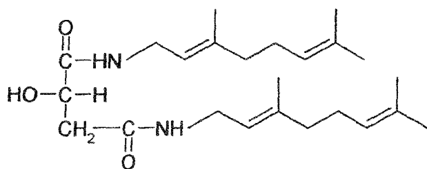
O-acetyl-N-geranylmalic monoamide
