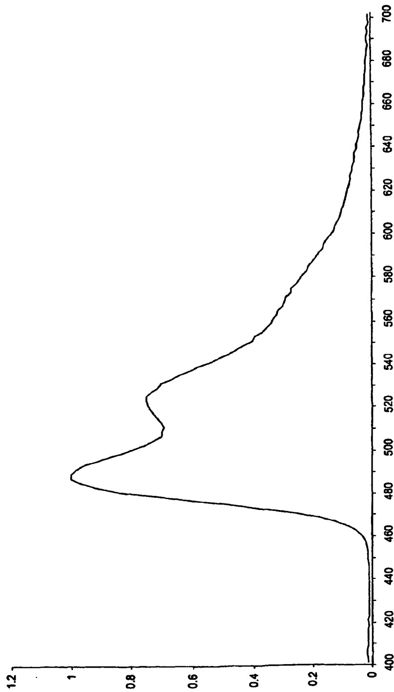
Figure 14. Emission spectrum of es101 in methylene chloride solution
